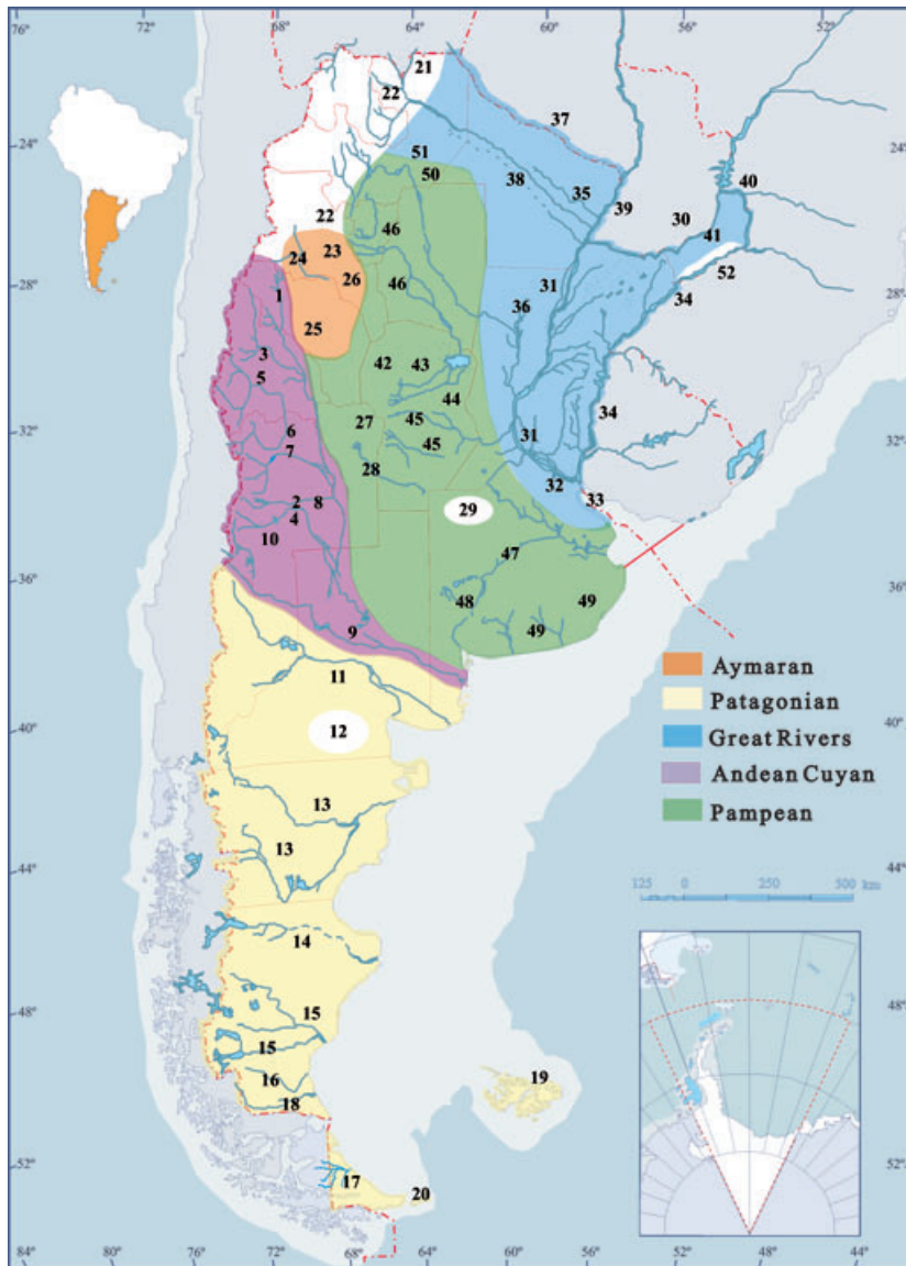
Figure 4 Ichthyological provinces of Argentina resulting from a parsimony analysis of endemicity (PAE) 50% majority-rule consensus tree of a matrix of 52 localities by 440 species. Numbers of localities correspond to lists in the text. Areas in white correspond to unresolved localities.
