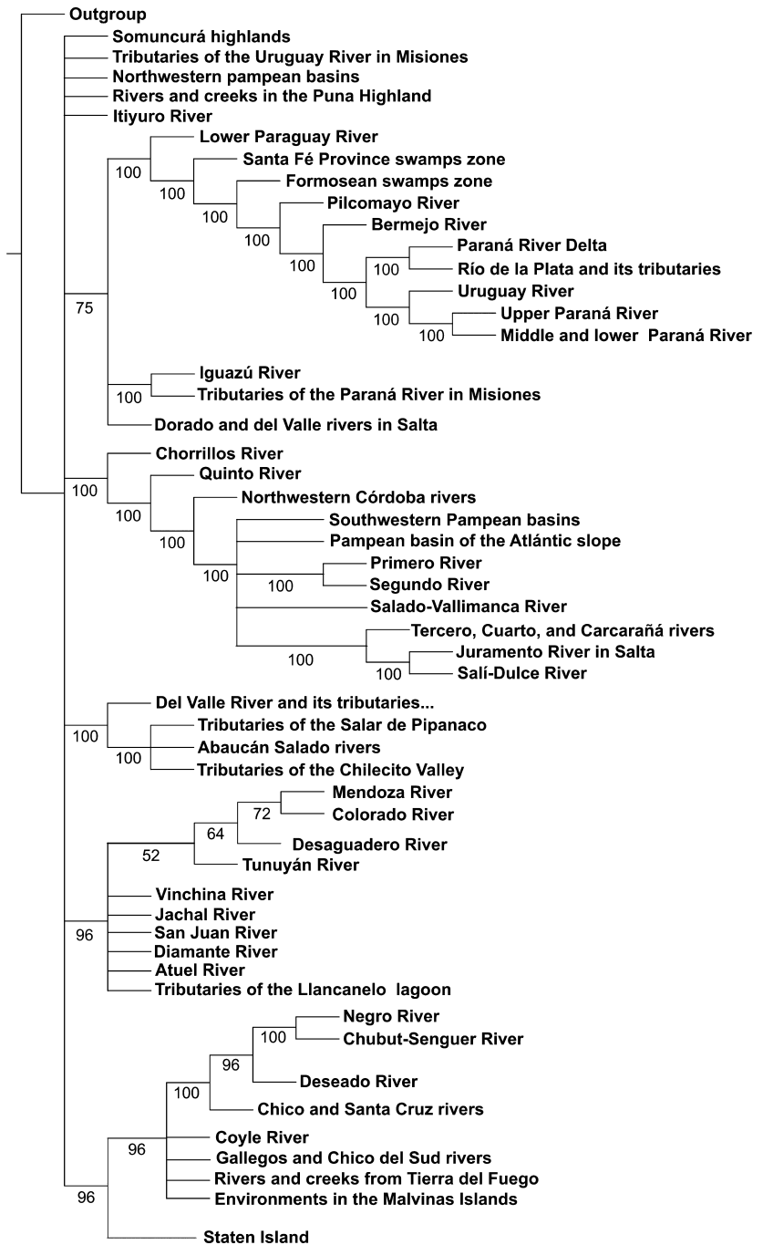
Figure 2 50% majority-rule consensus tree of 1196 trees (L = 1045; CI = 34; RI = 61) obtained from parsimony analysis of endemicity (PAE). Frequencies of occurrence are shown above the branches.
