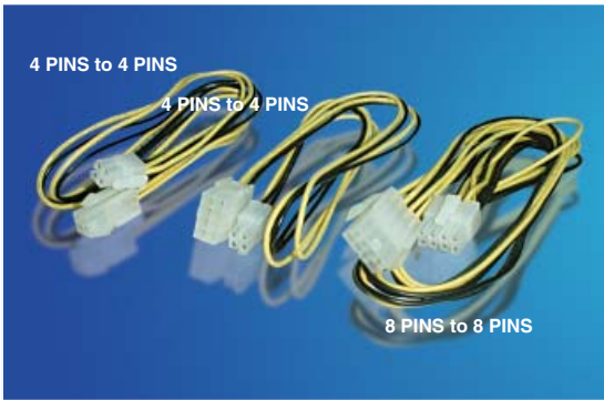
CLM-311111/311113/311115 P4 & Xeon CPU Expansion cables
