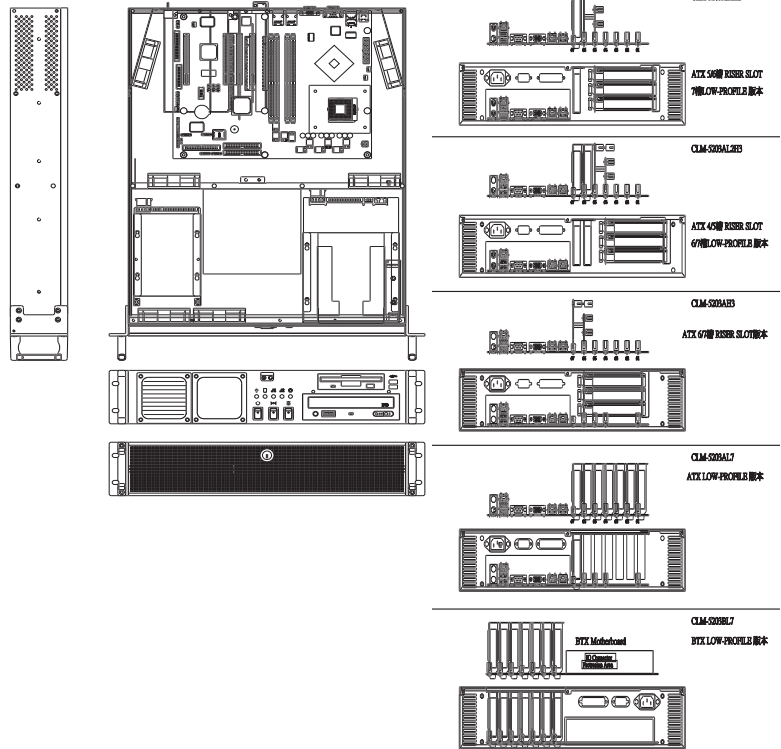
Constructon Drawing
