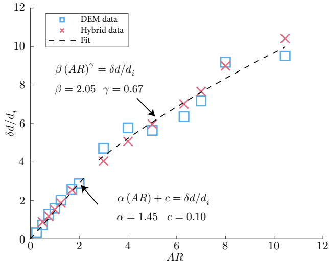
Fig. 6. Runout of a 2D granular column: Nondimensionalized runout distance, \delta d/d_i = (d_f - d_i)/d_i , vs aspect ratio, AR = h_i/d_i . Like DEM, our hybrid technique captures the two distinct regimes that Lube [2005] observed in experiments. We perform a linear fit in the low-AR regime, and a power-law fit in the high-AR regime.
