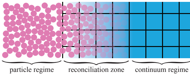
Fig. 3. Hybrid Reconciliation Zone as a Blurred Transition: A density partition applied to a partially discrete (left), partially continuum (right) system. Note that for simplicity, in the current study we set the densities to fixed values of 1/2 for each system throughout the reconciliation zone.
