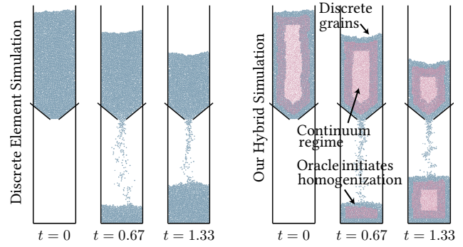
Fig. 8. Silo discharge: A silo discharges grains with a discrete method (left) and with our hybrid method (right).
