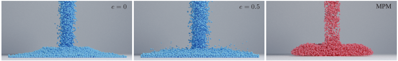
Fig. 11. Silo discharge (3D large orifice, r = 1.8 ): Our hybrid approach supports a range of restitution coefficients. Left: with 0 restitution, the flow looks uniform. Middle: with e = 0.5 , the flow appears more energetic, with multiple visible fly away grains. Observe that the MPM version of this simulation (right) has both a less energetic flow, and fails to simulate grains bouncing away from the bulk whole. The MPM counterpart is simulated with sticky boundary conditions on the bottom.
