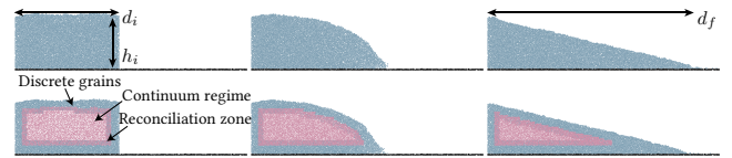
Fig. 5. Granular column: A collapsing column simulated with DEM (top) and with our hybrid approach (bottom). Observe the nice agreement in the final profile with our hybrid approach and the purely DEM approach.
