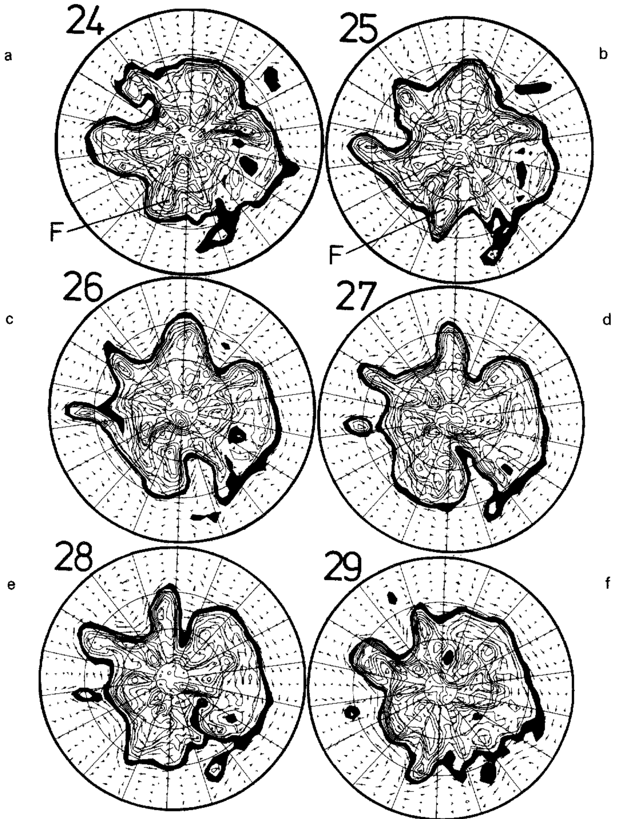
Figure 3. 330K IPV maps for the region north of 20^{\circ}\text{N} for the period 24–29 September 1982. The contour interval is 1.0PV units and the regions with values 1–2 units are blacked in. Also shown are the horizontal velocity vectors on this surface, scaled as in Fig. 2.
