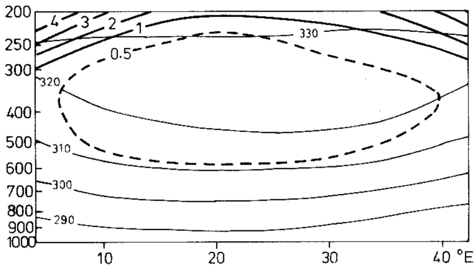
Figure 14. A vertical section on 4 October 1982 along the line at 60°N shown in the corresponding panel of Fig. 11. As in Fig. 9(a), the light continuous lines are isentropes drawn every 10 K and the heavy continuous lines are PV contours every 1 unit. The heavy dashed contour indicates a PV value of 0.5 units.
