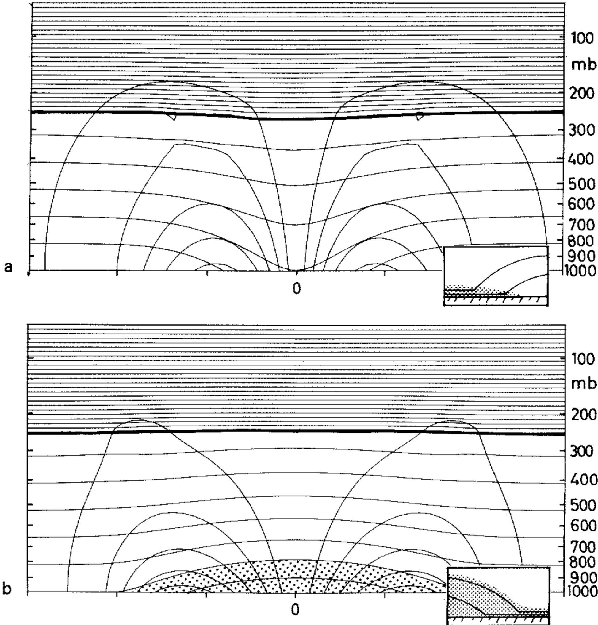
Figure 16.. Circularly symmetric flows induced by simple boundary temperature anomalies. The basic situation, and the method of solution, is as in Fig. 15 except that here there is no potential temperature variation along the tropopause, but the boundary potential temperature is taken to vary in the manner \frac{1}{2}A\{\cos(\pi\bar{r}/r_0) + 1\} for \bar{r} < r_0 = 1667 km. The amplitude A was taken to be +10 K in (a) and -10 K in (b). The thick line again represents the tropopause, and the thin lines the isentropes every 5 K and the transverse velocity every 3 \text{ m s}^{-1} . The zero isotach on the axis of symmetry is omitted. The warm anomaly induces a cyclonic circulation, and the cold anomaly an anticyclonic circulation. The surface pressure anomalies are -31 mb and +18 mb respectively, and the maximum (surface) winds are about 16 \text{ m s}^{-1} and 17 \text{ m s}^{-1} respectively. The relative vorticity extrema are at the surface and have values +0.8f and -0.5f respectively. The insets and stippling suggest the interpretation of the warm surface potential temperature anomaly as equivalent to a cyclonic IPV anomaly, and the cold surface potential temperature anomaly as part of an anticyclonic IPV anomaly (see text). For more details of the method of computation, see Thorpe (1985). Courtesy of A. J. Thorpe.
