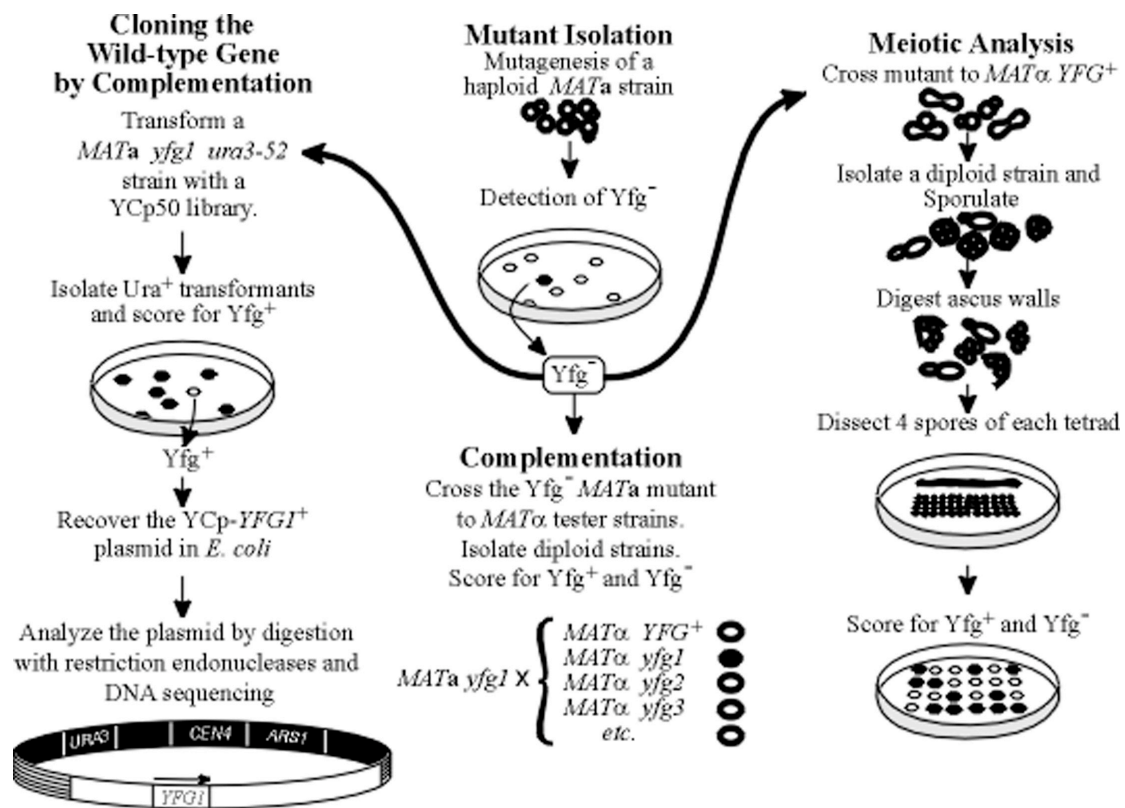
Figure 5.1. General approaches for genetic analysis. As an example, a MATa strain is mutagenized and a hypothetical trait, Yfg - (Your Favorite Gene) is detected. The Yfg - mutant is analyzed by three methods, complementation, meiotic analysis and molecular cloning (see the text).
