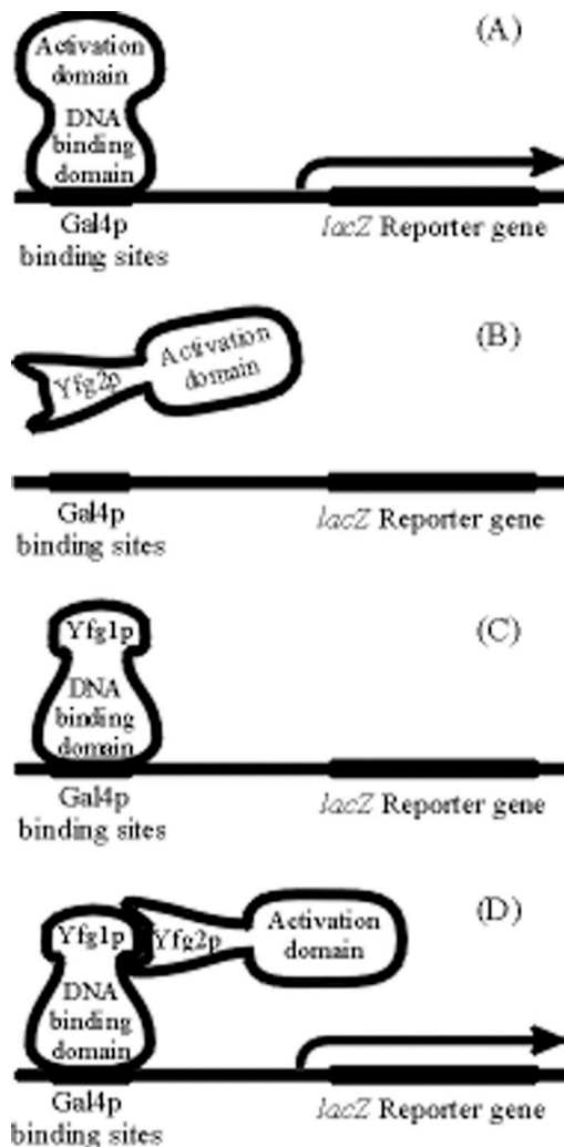
Figure 12.1. The two-hybrid system. (A) Normally, the Gal4 transcription activator binds to DNA at the Gal4p binding sites and activates transcription of the lacZ reporter gene. (B) A hybrid of the Gal4 activation domain with the Yfg2 protein does not activate transcription because it does not localize at the Gal4 binding site. (C) A hybrid of the Gal4 DNA-binding site domain with the Yfg1 protein does not activate transcription of the reporter gene because of the lack of the transcriptional activation domain. (D) Protein-protein interaction between Yfg1p and Yfg2p reconstitutes Gal4p function and activates transcription of the reporter gene.
