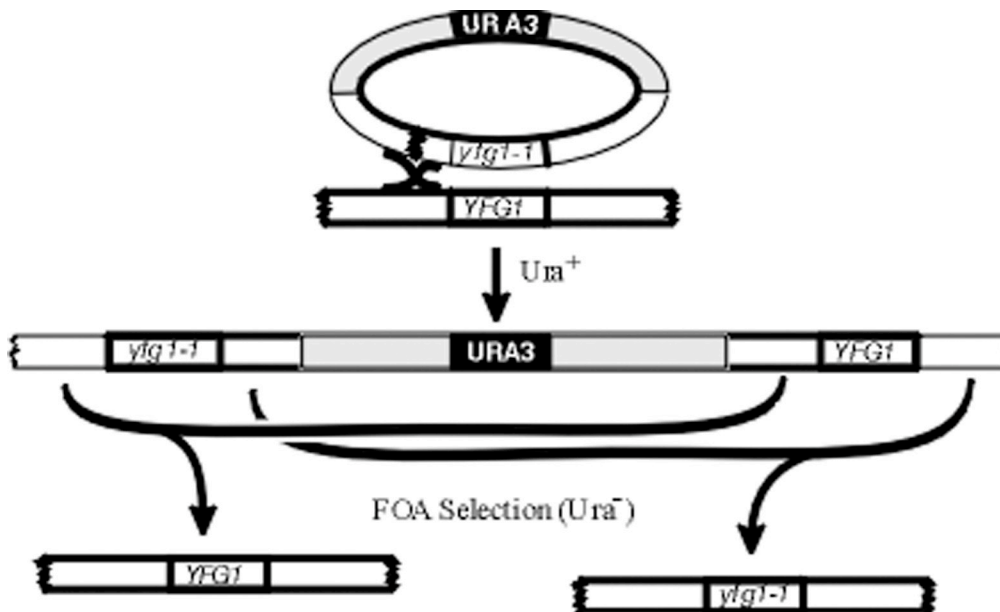
Figure 7.1. Two-step gene replacement. The wild-type chromosomal YFG1+ allele can be replaced by the mutant yfg1-1 allele from a YIp integrating plasmid. The plasmid is first integrated in the chromosome corresponding to the site on the plasmid that was cleaved by a restriction endonuclease. Strains that have excised the URA3 marker in vivo by homologous recombination are selected on FOA medium. Either the original YFG1+ allele, or the yfg1-1 allele remains in the chromosome, depending on the site of the cross-over.
