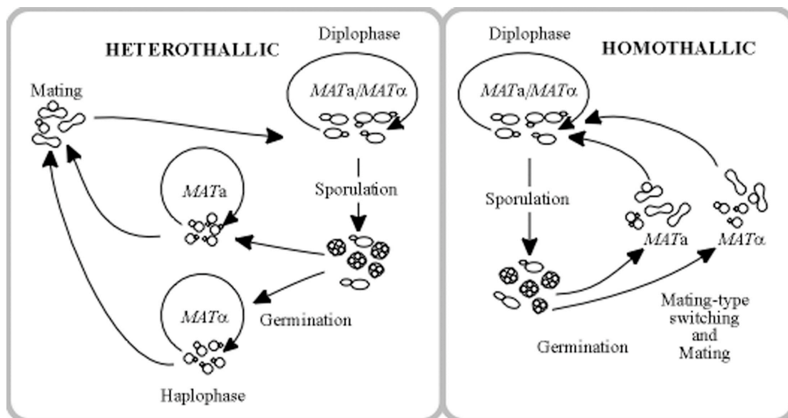
Figure 2.1. Life cycles of heterothallic and homothallic strains of S. cerevisiae . Heterothallic strains can be stably maintained as diploids and haploids, whereas homothallic strains are stable only as diploids, because the transient haploid cells switch their mating type, and mate.
