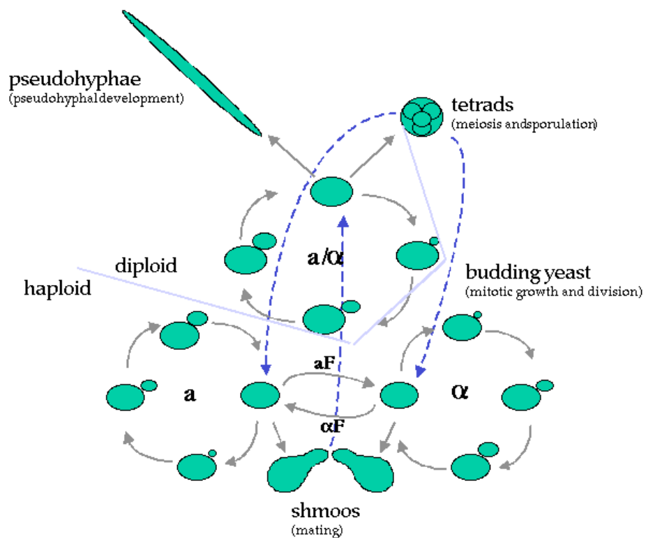
Figure 2.2. Life cycles of heterothallic and homothallic strains of S. cerevisiae .
