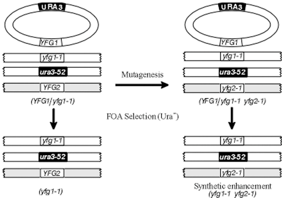
Figure 10.1. Synthetic enhancement and synthetic lethality. Novel chromosomal genes mutations, yfg2-1 , etc., that enhance the phenotype of a yfg1-1 mutations can be uncovered by mutagenizing a yfg1-1 strain containing a YCp plasmid p[ YFG1 URA3 ], and subsequently selecting for the loss of the plasmid. If yfg1-1 yfg2-1 strain are inviable, they will not grow on FOA medium.
