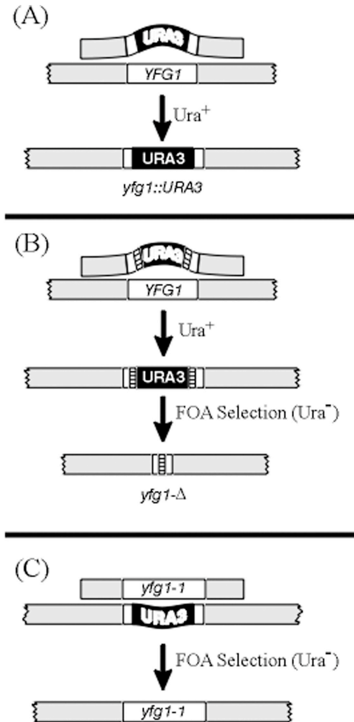
Figure 9.2. Gene disruption and single-step gene replacement. (A) The YFG1 + gene is disrupted by transforming the strain with a linear fragment containing a URA3 selectable marker flanked by homologous sequences. The chromosomal segment is replaced by this URA3 containing fragment after integration by homologous recombination at the two ends. (B) The URA3 marker introduced in the YFG1 locus, can be excised if URA3 is also flanked by direct repeats of DNA, preferably not originating from yeast. Homologous recombinants, selection on FOA medium, lack
