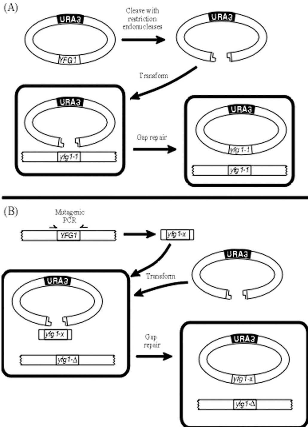
Figure 9.1. (A) Retrieval of a chromosomal yfg1-1 mutation by transforming a mutant with a gapped plasmid. Only the repaired circular plasmid containing the mutation is stably maintained in yeast. (B) Generation of a series of yfg1-x mutations by PCR mutagenesis and gap repair. The yfg1-Δ mutant is cotransformed with the mutagenized PCR fragments and the gapped plasmid. The phenotypes of the yfg1-x mutants can be directly assessed in the strain containing the yfg1-Δ deletion.
