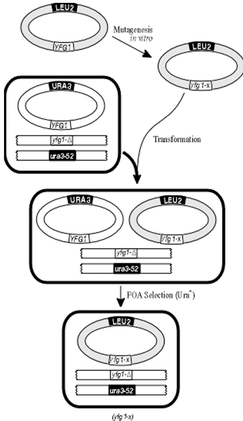
Figure 9.3. Plasmid shuffle. The chromosomal copy of YFG1 is replaced by the yfg1-Δ deletion, but the Yfg + phenotype is maintained by the YCp plasmid containing YFG1 and URA3 . The strain is transformed with a mutagenized LEU2 plasmids having the YFG1 gene. Recessive yfg1-x mutations are manifested by selecting for strains on FOA medium. The strain will not grow on FOA medium if YFG1 is an essential gene and if the yfg1-x mutation is not functional.
