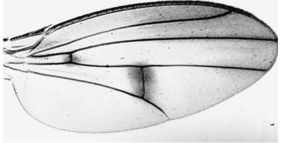
sclerstyla
