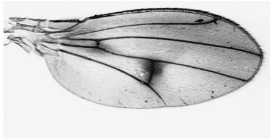
dextra
