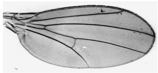
armata
