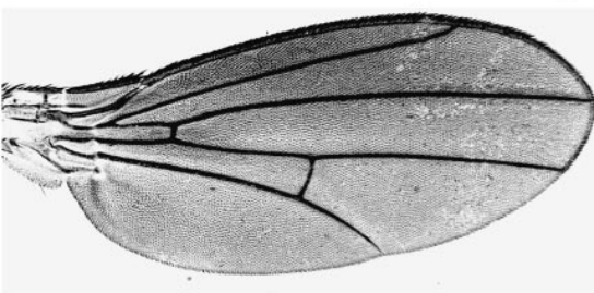
yanomama
