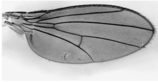
carinata
