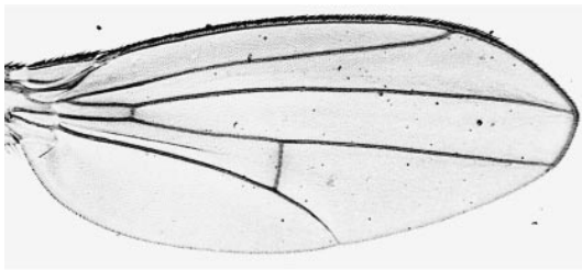
amblyharpa
