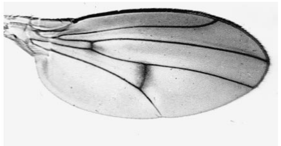
genuinus
