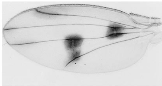
ranhyae
