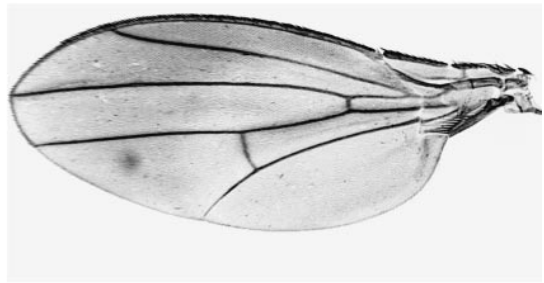
unca
