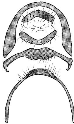
propenicula
