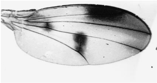
dominicana
