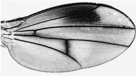
abbrevifusca
