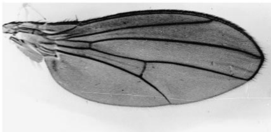
neosimplex
