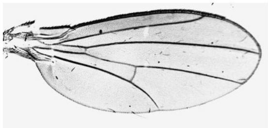
chelifera
