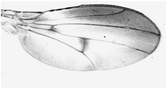
floridana
