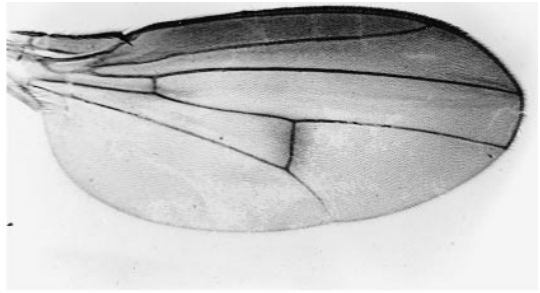
dracula
