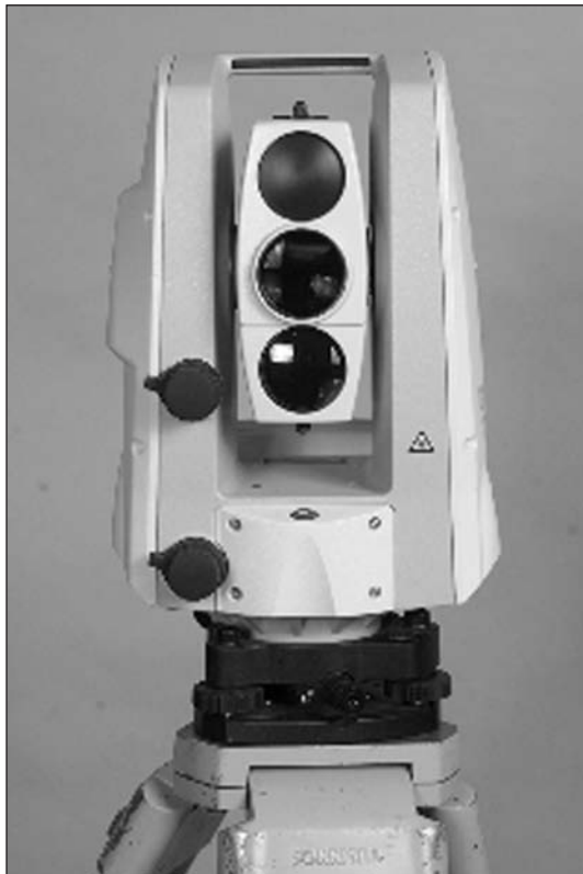
Figure D-1 Trimble TTS500 reflectorless total station.
