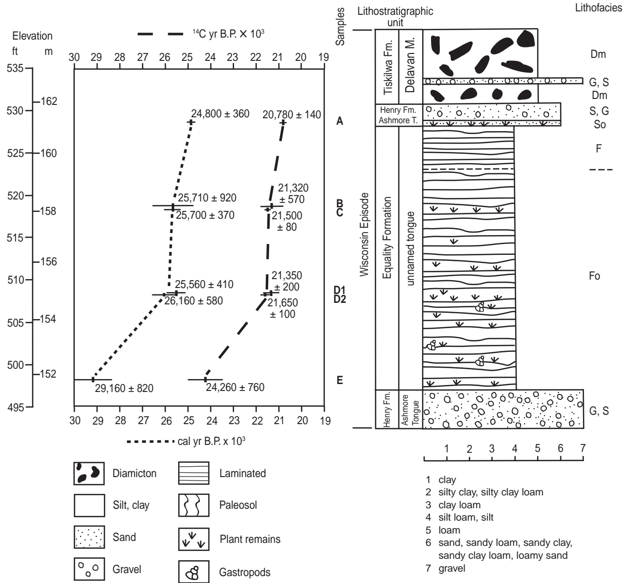
Figure 40 Lithostratigraphy and lithofacies interpretations and radiocarbon ages ( ^{14}\text{C} yr B.P. and cal yr B.P.) of deposits sampled in Core I-1081, located 600 m (1,968.5 ft) northeast of the outcrop at Stop 2-1. Lithofacies code is given in Figure 11.
