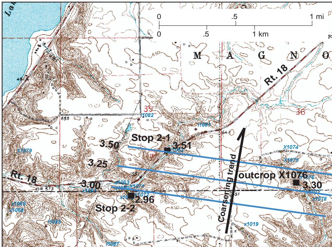
Figure 39 Contoured average values of the ratio of medium silt (16 to 31 \mu m) to fine silt (8 to 16 \mu m) for samples of late Wisconsin Episode loess (Morton Tongue) at three sites east of the Illinois River, Henry 7.5-minute Quadrangle.
