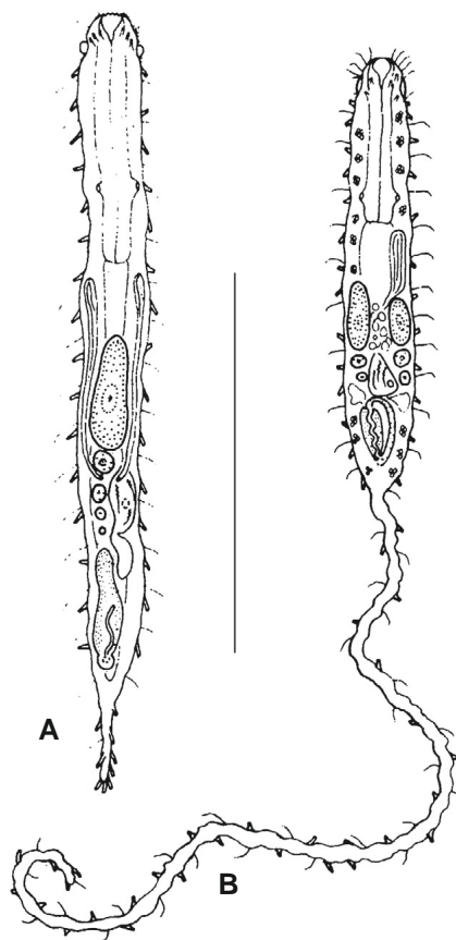
Fig. 6. Macrodasysida, Macrodasysidae – Representatives of the genera Macrodasys (A), Urodasys (B). Scale bar = 200 \mu m. A, B, modified from Ruppert (1988).
