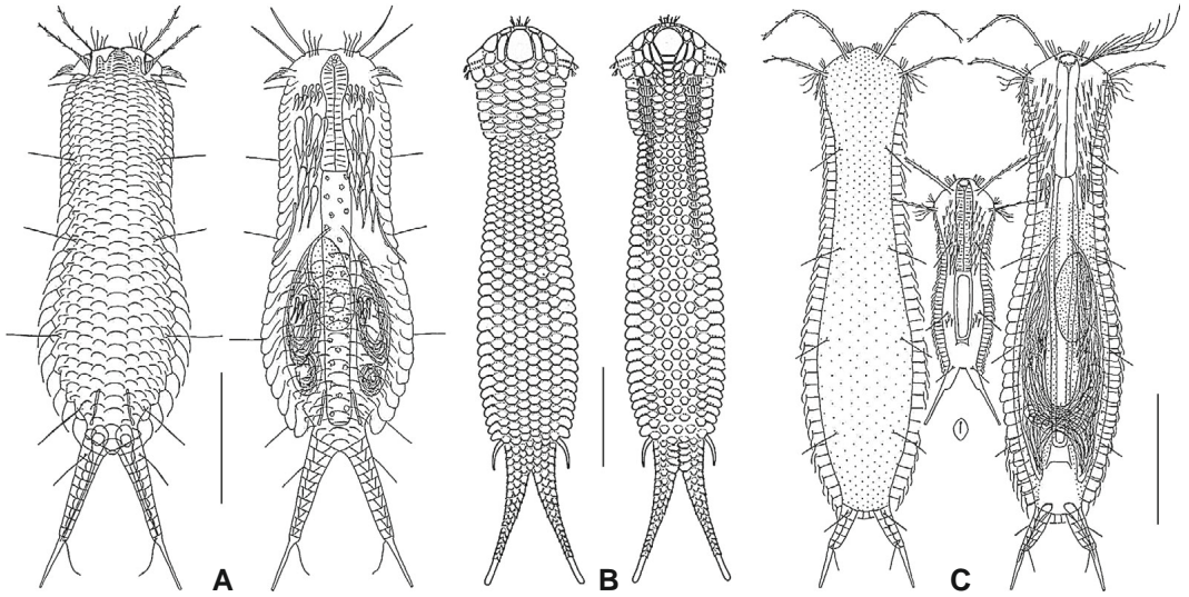
Fig. 10. Chetonotida, Xenotrichulidae – Representatives of the genera Heteroxenotrichula (A), Draculiciteria (B), Xenotrichula (C). Scale bars = 50 µm. A, C, original (W. D. Hummon); B, modified from Luporini et al. (1973).
