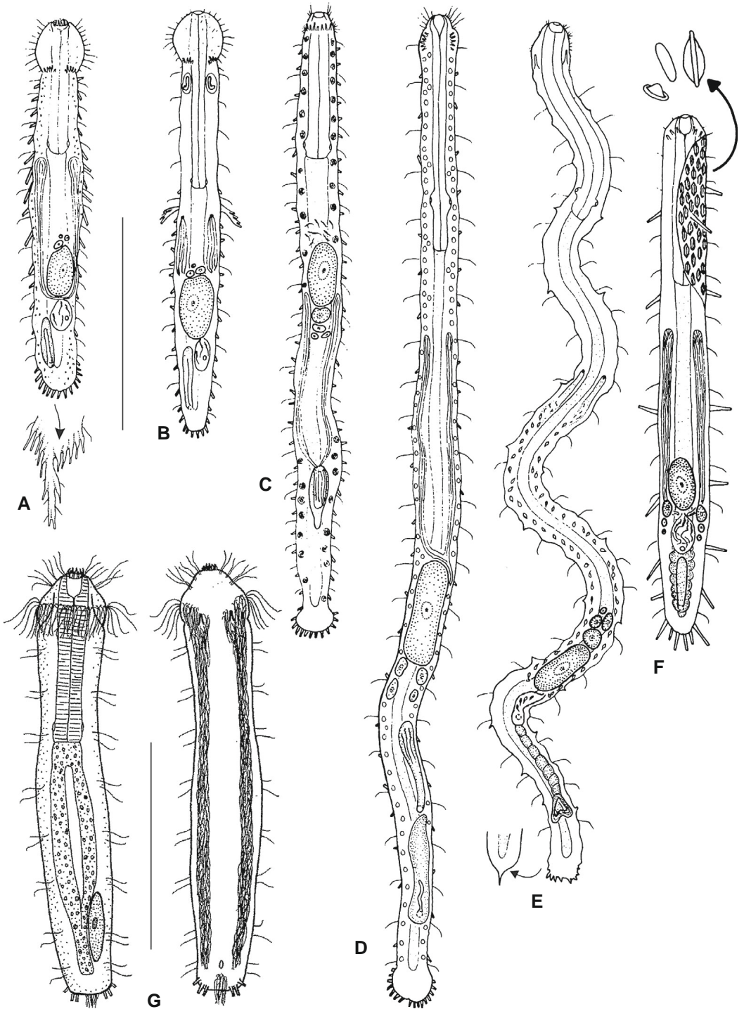
Fig. 4. Macrodasysida, Lepidodasysidae – Representatives of the genera Cephalodasys (A), Pleudodasys (B), Mesodasys (C), Megadasys (D), Dolichodasys (E), Lepidodasys (F), Paradasys (G). Scale bar = 200 \mu m. A-F, modified from Ruppert (1988); G, original (W. D. Hummon).
