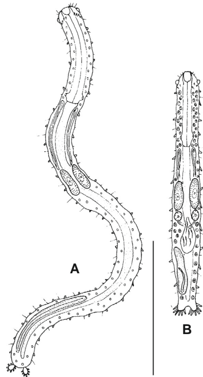
Fig. 8. Macrodasysida, Planodasyidae – Representatives of the genera Planodasys (A), Crasiella (B). Scale bar = 200 µm. A, B, modified from Ruppert (1988).
