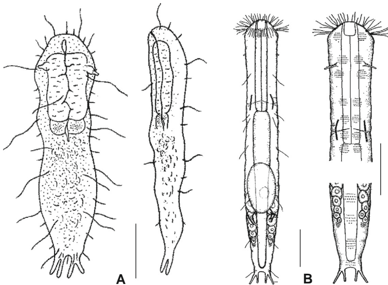
Fig. 9. Incertae sedis – Representatives of the genera Marinellina (A), Redudasys (B). Scale bars = 50 µm. A, Modified from Ruttner-Kolisko (1955); B, modified from Kisielewski (1987).
