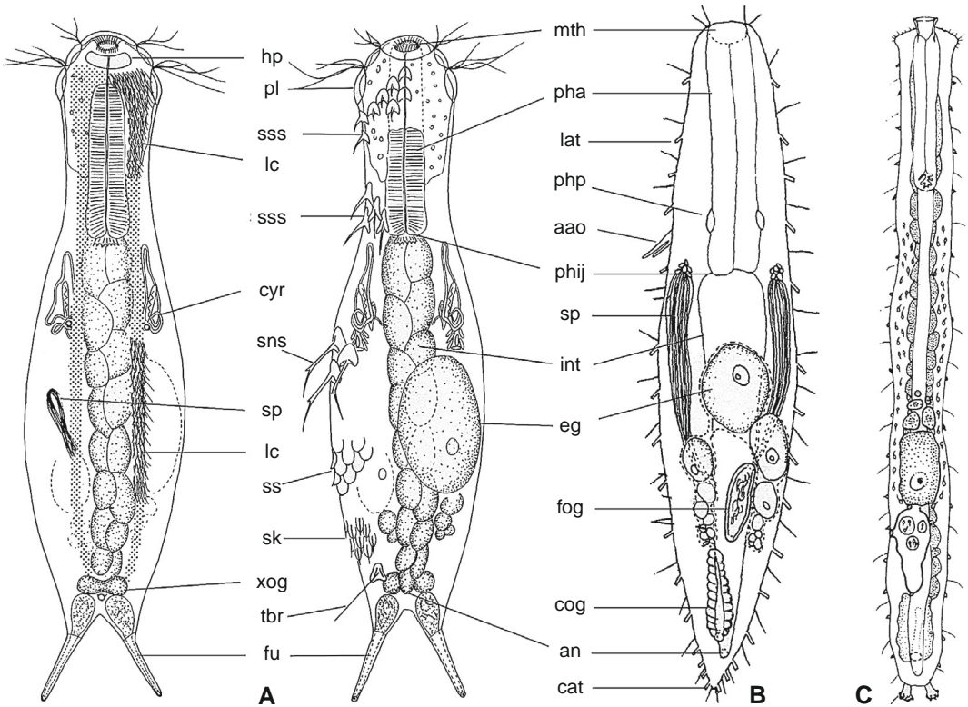
Fig. 1. A. Drawing of a hypothetical Chaetonotida Paucitubulatina. B. Drawing of a hypothetical Macrodasysida. C. Neodasys (Chaetonotida, Multitubulatina). Aao , accessory adhesive organs; an , anus; cat , caudal adhesive tubes; cog , caudal organ; cyr , cyrtocytes; eg , egg; fog , frontal organ; fu , furca; hp , hypostomion; int , intestine; lat , lateral adhesive tubes; lc , locomotor cilia; mth , mouth; pha , pharynx; phij , pharyngo-intestinal junction; php , pharyngeal pores; pl , pleuria; sk , keeled scale; sns , scales with notched spines; sp , sperm; ss , smooth scales; sss , scales with simple spines; tbr , tactile bristle; xog , X-organ. A, B , modified from Balsamo & Todaro (2003); C , Modified from Ruppert (1988).
