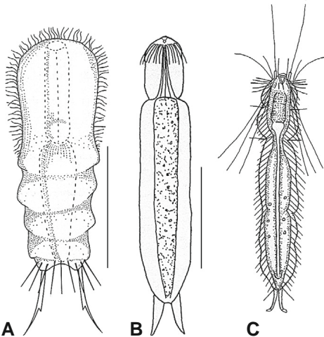
Fig. 11. Chetonotida: A, Dichaeturidae – Representative of the genus Dichaetura , B, C, Proichthydiidae – Representatives of the genera Proichthydiium (B), Proichthydioides (C). Scale bars = 50 µm. A, modified from Balsamo (1983); B, modified from Cordero (1918); C, Redrawn from Suzuki (1971).
