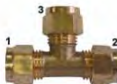
Tee pieces 1 x 2 x 3 1/4" x 1/4" x 1/4" 070068 5/8" x 5/8" x 5/8" 070074 3/8" x 3/8" x 3/8" 070079 5/8" x 5/8" x 1/4" 070081 8 x 8 x 8mm 070080 8 x 10 x 8mm 070083 10 x 10 x 8mm 070085 15 x 15 x 10mm 070087 15 x 15 x 8mm 070089
