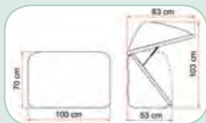
Ultra-box 320 12kg. 320 litre capacity 102256
