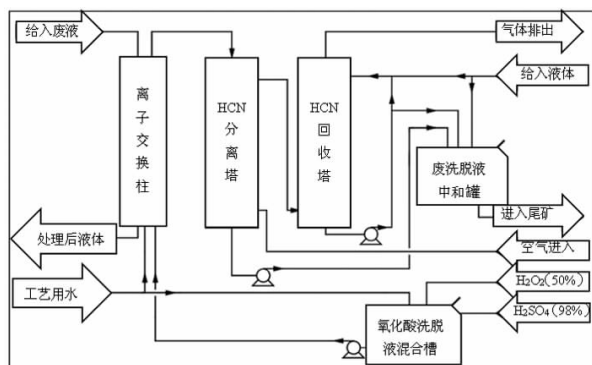
图 2 离子交换树脂处理氰化尾渣简化流程 [24] Fig. 2 Simplified flowchart of the ion exchange resin for cyanidation tailing treatment [24]
