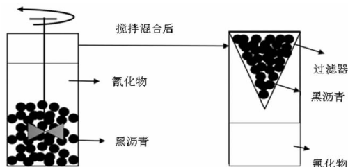
图 3 天然沥青去除氰化物溶液试验示意图 [24] Fig. 3 Schematic picture of cyanide solution removal by using natural asphalt tests [24]
