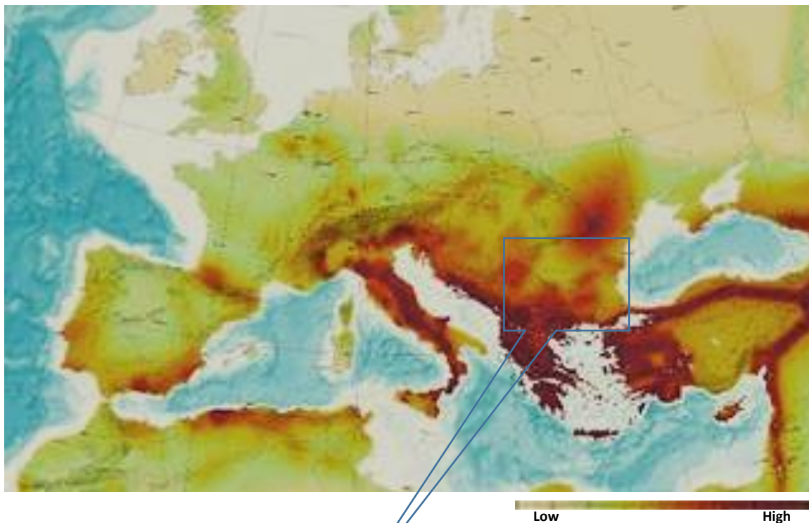
Map 11: Map of seismic hazard in Europe
