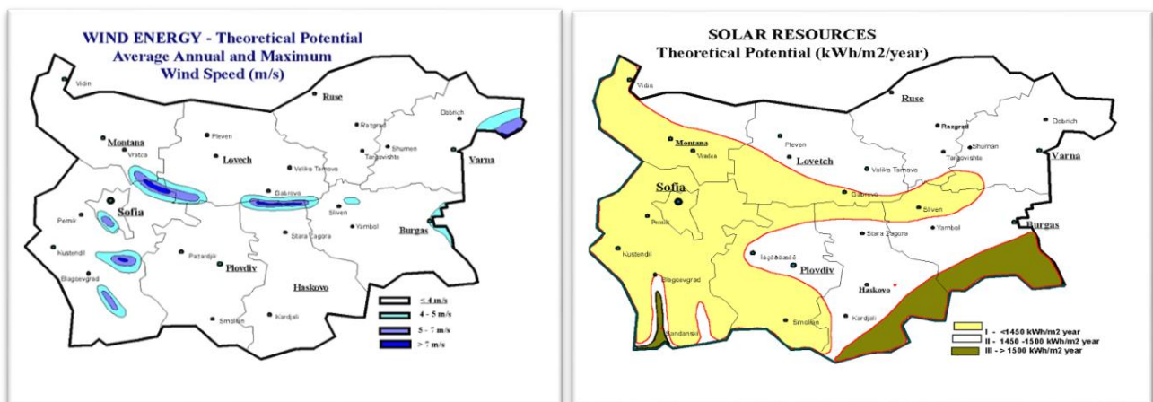
Map 20, Map 21: Maps of Wind energy and Solar resources in Republic of Bulgaria
