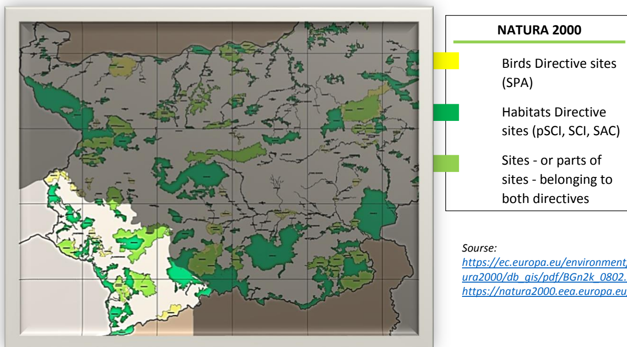
Map 4: Natura 2000 sites in Republic of Bulgaria
