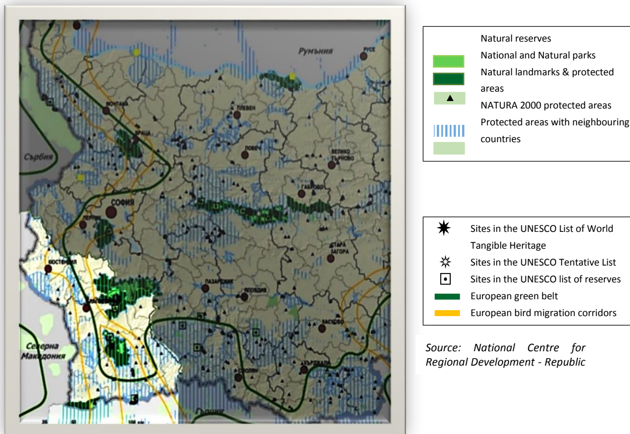
Map 23: Natural Heritage in CBC region of the Republic of Bulgaria
