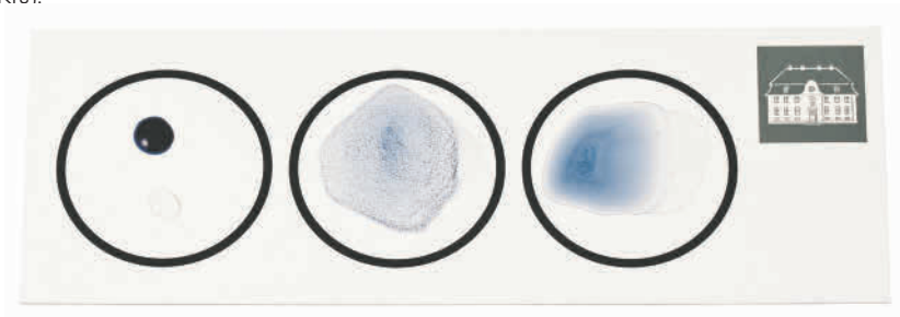
Figure 6. Latex agglutination – To the left a drop of latex and bacterial suspension. In the middle a positive agglutination, and a negative agglutination to the right.
