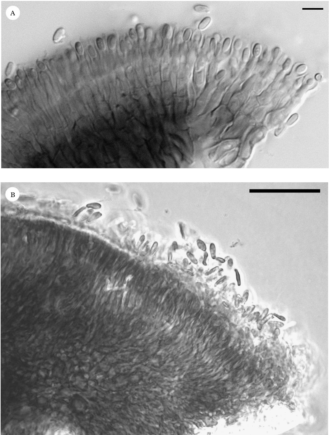
FIG. 3. Lambinonia strigulae . A, section through a sporodochium showing conidiophores and conidiogenesis (A. Vězda 24 vi 1979); B, section through a sporodochium covered by numerous conidia (J. Lambinon 72-959) (in water, phase contrast). Scales: A=10 \mu m; B=20 \mu m.
