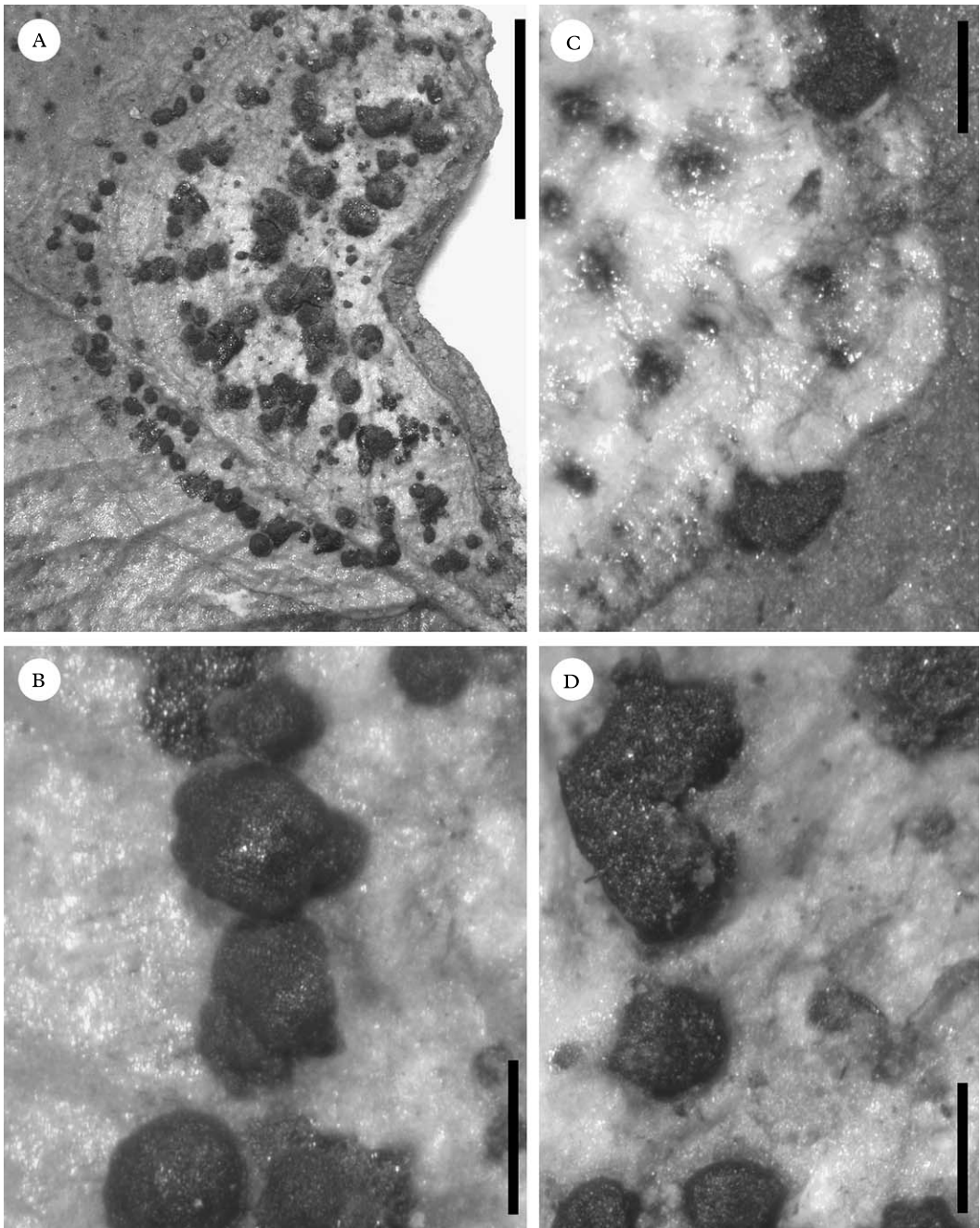
FIG. 1. Lambinonia strigulae . A, thallus of Strigula nitidula with numerous concentrically arranged sporodochia (neotype, BRA: A. Vězda, 17 vi 1978); B, same specimen, showing strongly convex sporodochia; C, thallus of S. buxi with two marginal, flattened sporodochia (D. Puntillo 10390); D, thallus of S. nemathora with slightly flattened sporodochia with a constricted base (visible in section, see Fig. 2A) ( J. Lambinon 72-959). Scales: A=1 mm; B-D=200 \mu m.
