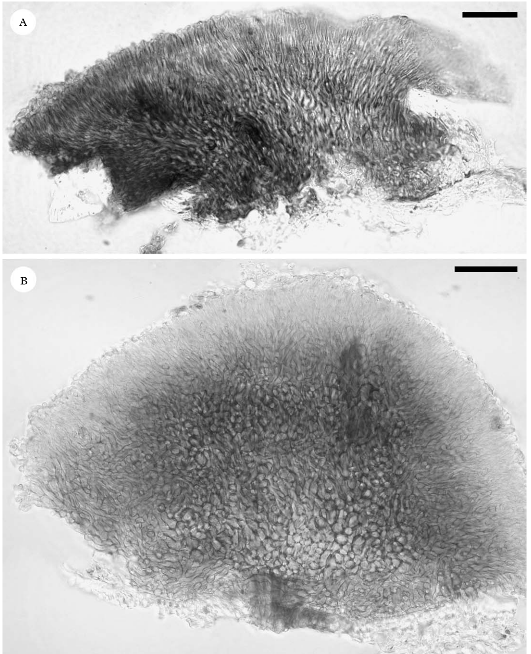
FIG. 2. Lambinonia strigulae . A, section through a blackish, slightly flattened sporodochium with a constricted base, on Strigula nemathora (f. Lambinon 72-959) (in lactophenol cotton blue); B, section through a greyish, strongly convex sporodochium, on S. buxi (A. Vězda, 15 vi 1979) (in water). Scales: A & B=20 \mu m.
