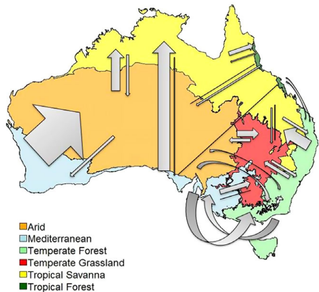
Figure 5. Inferred shifts among Australian biomes during the diversification of Hakea . Width of the arrows is proportional to the relative number of inferred shifts under the BAYAREA + J + X model.
