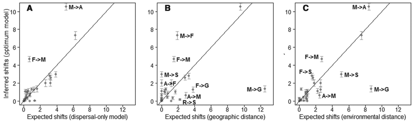
Figure 4. Inferred and expected numbers of shifts between each pair of biomes during the diversification of Hakea .
