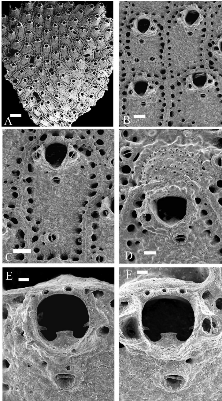
Figure 16. Smittoidea reginae . Hassler Box 15. MCZ 100124. A. Encrusting colony fragment. Scale bar = 500 \mu\text{m} . B. Four autozooids. Scale bar = 100 \mu\text{m} . C. Close-up of a single autozooid, showing three avicularia around the peristome and a single proximal avicularium. Scale bar = 100 \mu\text{m} . D. Ovicelled zooid. Scale bar = 100 \mu\text{m} . E. Close-up of an orifice with two distal spines. Scale bar = 20 \mu\text{m} . F. Another orifice with three distal spines. Scale bar = 20 \mu\text{m} .
