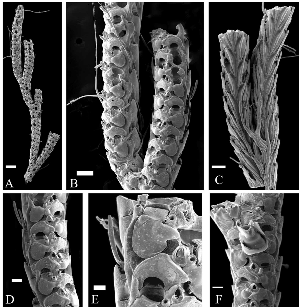
Figure 9. Caberea hassleri-1 . Hassler Box 5. MCZ 100117. A. Low magnification view of large branch fragment to show branch form and branching pattern. Scale bar = 500 \mu\text{m} . B. Two branches showing morphology of zooids, scuta, and ovicells. Scale bar = 250 \mu\text{m} . C. Abfrontal surface of branch. Scale bar = 100 \mu\text{m} . D. Portion of a branch showing small avicularia and spines. Scale bar = 100 \mu\text{m} . E. Close-up of growing tip of branch. Scale bar = 20 \mu\text{m} . F. Giant avicularium on branch. Scale bar = 100 \mu\text{m} .
