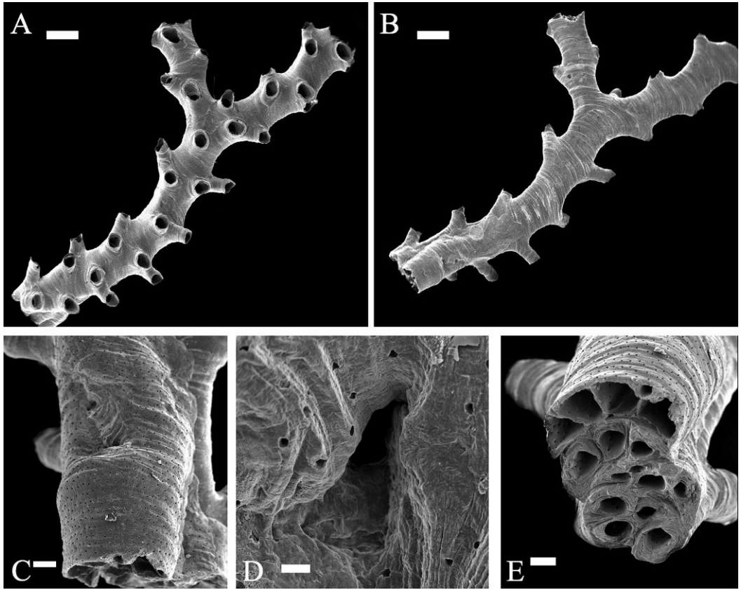
Figure 5. Tervia sp. Hassler Box 7. MCZ 100113. A. Frontal view of colony branch. Scale bar = 500 µm. B. Abfrontal surface of same branch. Scale bar = 500 µm. C. Possible gonozooid. Scale bar = 100 µm. D. Opening to possible gonozooid. Scale bar = 20 µm. E. View of broken proximal end of branch. Scale bar = 100 µm.
