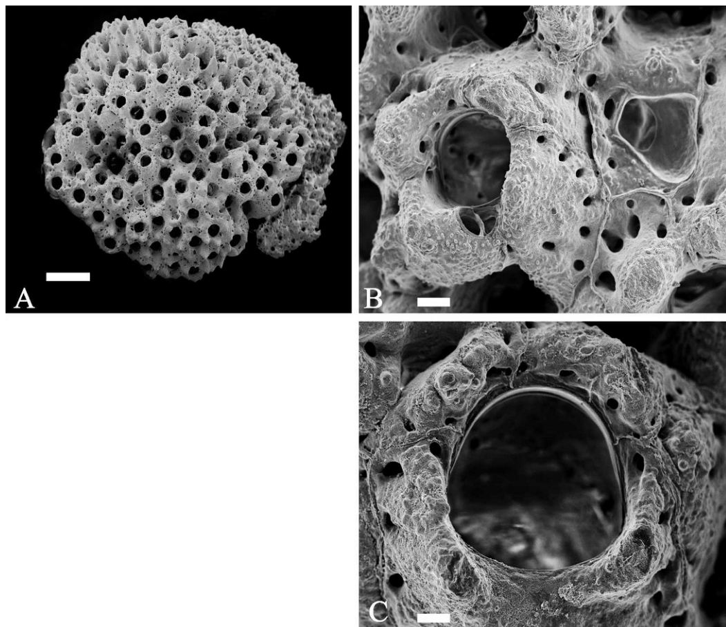
Figure 33. Trematoeocia turrita . Box 1-2. MCZ 100141. A. Whole nodular colony. Scale bar = 1 mm. B. Zooid with peristomial avicularium and adjacent spatulate interzoocelial avicularium. Scale bar = 100 \mu m. C. Close-up of orifice. Scale bar = 50 \mu m.
