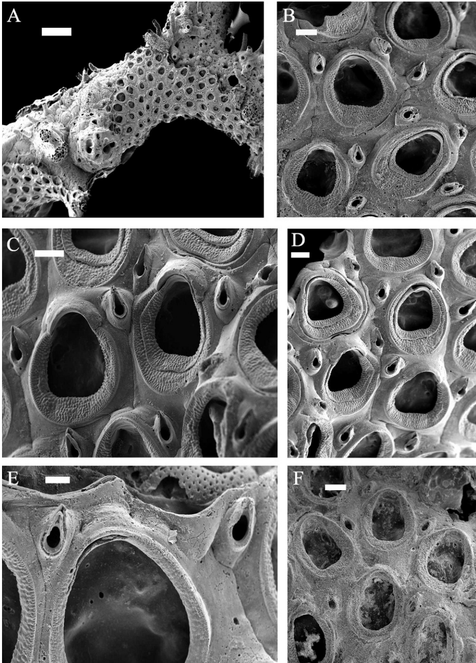
Figure 7. Antropora typica-1 . (A–E Hassler Box 6. MCZ 10016) A. Entire colony attached to calcareous substratum. Scale bar = 1 mm. B. Group of zooids and avicularia at growing edge of colony. Scale bar = 100 \mu m. C. Two ovicelled zooids. Scale bar = 100 \mu m. D. Another group of zooids and avicularia. Scale bar = 100 \mu m. E. Close-up of two avicularia at growing edge of colony. Scale bar = 50 \mu m. F. (Hassler Box 2. MCZ 10015) Zooids and avicularia from another colony. Scale bar = 100 \mu m.
