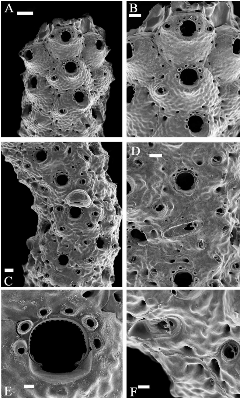
Figure 35. Stephanollona propinqua-1 . Hassler Box 14. MCZ 100143. A. Growing tip of colony encrusting a tubular substratum. Scale bar = 200 \mu\text{m} . B. Zooids at growing edge, showing oral spines and early avicularian development. Scale bar = 100 \mu\text{m} . C. Portion of colony showing ovicelled zooid with double pairs of avicularia. Scale bar = 100 \mu\text{m} . D. Area of colony with many small avicularia and one larger elongate oval avicularium. Scale bar = 100 \mu\text{m} . E. Close-up of an orifice with six spines; note beaded rim, and double-ended condyles. Scale bar = 25 \mu\text{m} . F. Large avicularium with bent and pointed rostrum and small, almost round, avicularium. Scale bar = 50 \mu\text{m} .
