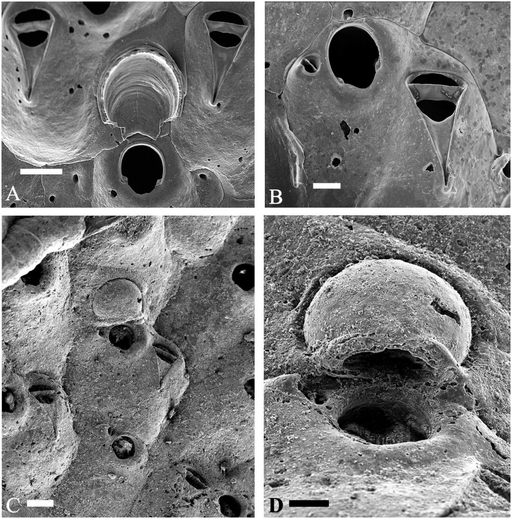
Figure 30. Buffonellaria ensifera-2 . (A-B Hassler Box 15. MCZ 100137) A. Giant avicularia and developing ovicell. Scale bar = 100 \mu\text{m} . B. An autozooid with both types of avicularia. Scale bar = 50 \mu\text{m} . (C-D Hassler Box 2. MCZ 100138) C. Ovicelled zooid. Scale bar = 100 \mu\text{m} . D. Close-up of ovicell. Scale bar = 50 \mu\text{m} .
