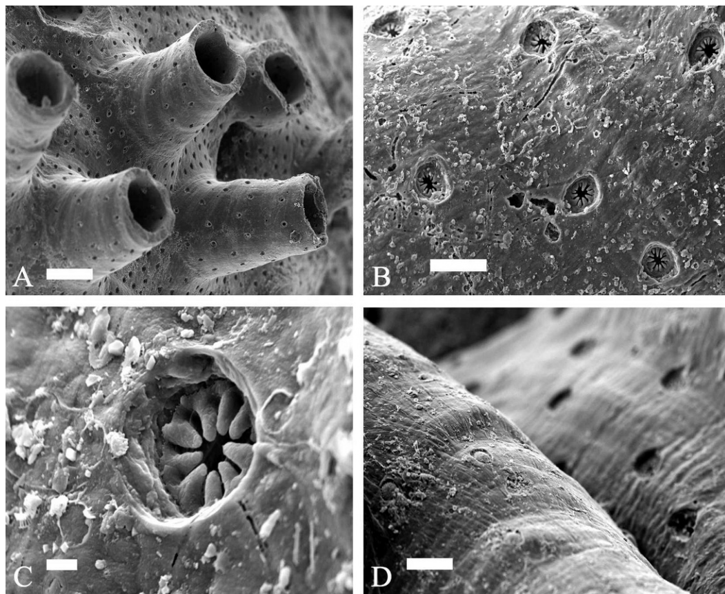
Figure 4. Proboscina robusta-2 . A. Close-up of pores on zoid peristomes and colony surface. Scale bar = 100 \mu m. B. Magnified view of pores showing radial denticles. Scale bar = 10 \mu m. C. Highly magnified pore. Scale bar = 1 \mu m. D. Direct comparison of pore structure of Stomatopora (on left) and Proboscina (on right) zooids. Scale bar = 10 \mu m.
