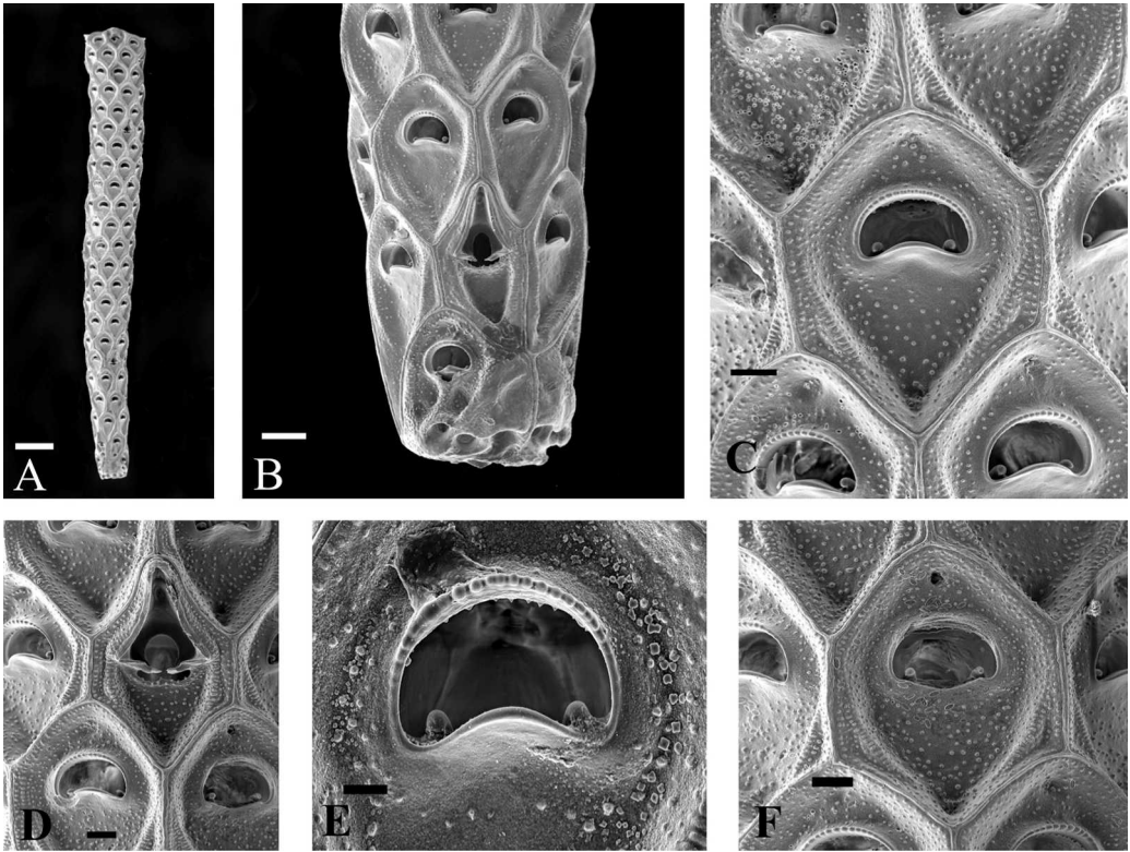
Figure 13. Cellaria louisorum . Hassler Box 3. MCZ 100120. A. One branch internode. Scale bar = 500 \mu\text{m} . B. Close-up of proximal end of internode showing avicularium and zooids. Scale bar = 100 \mu\text{m} . C. An autozoid. Scale bar = 100 \mu\text{m} . D. Close-up of an avicularium. Scale bar = 50 \mu\text{m} . E. Close-up of orifice, showing beaded distal rim, curved proximal rim, and rounded condyles. Scale bar = 20 \mu\text{m} . F. Fertile zoid, showing ovicell foramen and wider orifice. Scale bar = 50 \mu\text{m} .
