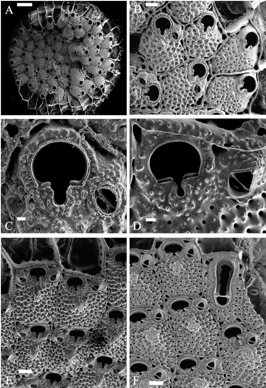
Figure 22. Stylopoma smitti and Stylopoma haywardi . (A–C, S. smitti , Hassler Box 1-2, MCZ 100130.) A. Entire juvenile colony. Scale bar = 500 \mu\text{m} . B. Group of autozooids at growing edge of colony. Scale bar = 100 \mu\text{m} . C. Distal end of autozooid of same colony showing orifice shape and small frontal avicularium. Scale bar = 200 \mu\text{m} . (D–F, S. haywardi , Hassler Box 1-1, MCZ 100131.) D. Orifice of zooid from second colony to show orifice shape and morphology of frontal avicularium. Scale bar = 20 \mu\text{m} . E. Group of autozooids of this colony near growing edge. Scale bar = 100 \mu\text{m} . F. Another group of zooids showing large spatulate interzoocelial avicularium. Scale bar = 100 \mu\text{m} .
