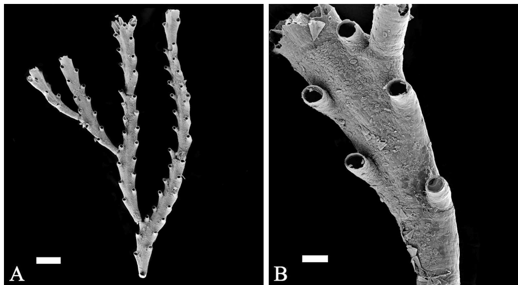
Figure 1. Crisia sp. Hassler Box 4. A. Branches of colony. Scale bar = 500 \mu\text{m} . B. Zooids, showing size of tubes and orifice shape. Scale bar = 100 \mu\text{m} . MCZ 100108.
