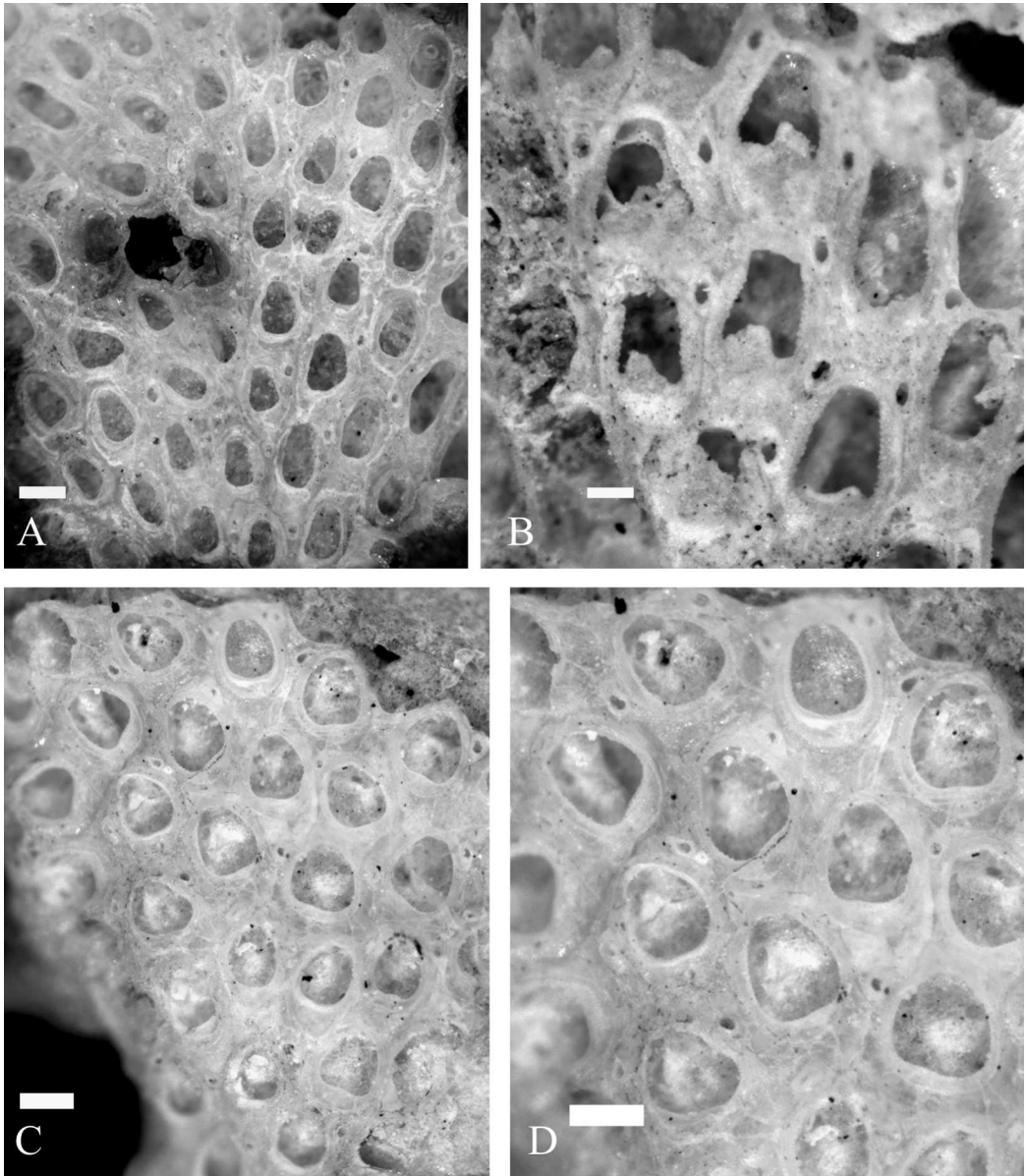
Figure 8. Antopora typica -2. Light micrographs of type material of Canu and Bassler. A. Dacryonella typica USNM 7484 cotype 1. Scale bar = 200 \mu m. B. Dacryonella typica . Magnified view of zooids and avicularia. USNM 7484 cotype 2. Scale bar = 100 \mu m. C. Membrendoecium strictorostriis . Type. USNM no. 7552. Scale bar = 200 \mu m. D. Membrendoecium strictorostriis . View of several zooids at higher magnification, same specimen. Scale bar = 200 \mu m.
