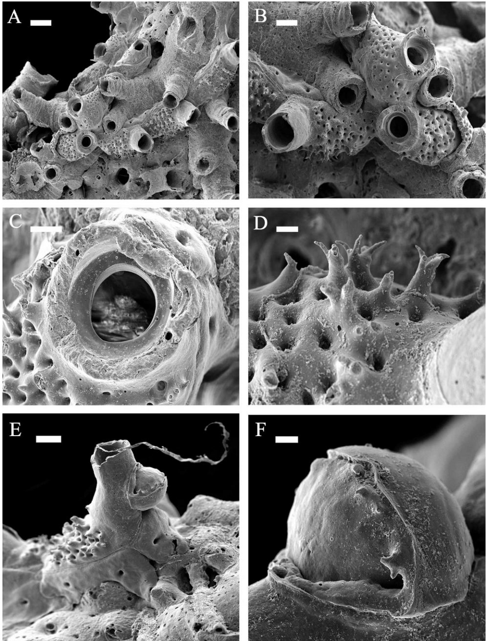
Figure 25. Lagenicella verrucosa . Hassler Box 6. MCZ 1000133. A. Lagenicella colony intertwined with cyclostome colony ( Proboscina ). Scale bar = 200 \mu m. B. Three Lagenicella zooids and adjacent cyclostome zooids. Scale bar = 100 \mu m. C. Orifice (near level of primary orifice and developing peristome). Scale bar = 50 \mu m. D. Spiny and knobby calcified projections on frontal shield. Scale bar = 20 \mu m. E. Ovicelled zooid in side view. Scale bar = 100 \mu m. F. Close-up of ovicell. Scale bar = 20 \mu m.
