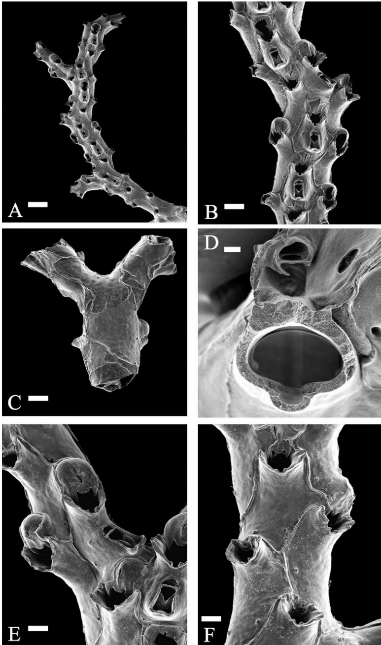
Figure 37. Reteporellina directa-1 . Hassler Box 13. MCZ 100144. A. Colony branches. Scale bar = 500 \mu\text{m} . B. Close-up of branch, showing zooid morphology and position and orientation of avicularia. Scale bar = 200 \mu\text{m} . C. Back view of branch at a bifurcation. Scale bar = 200 \mu\text{m} . D. Partial view of primary orifice. Scale bar = 20 \mu\text{m} . E. Ovicelled zooids at a branch bifurcation. Scale bar = 100 \mu\text{m} . F. Zooids without avicularia; two with ovicells. Scale bar = 100 \mu\text{m} .
