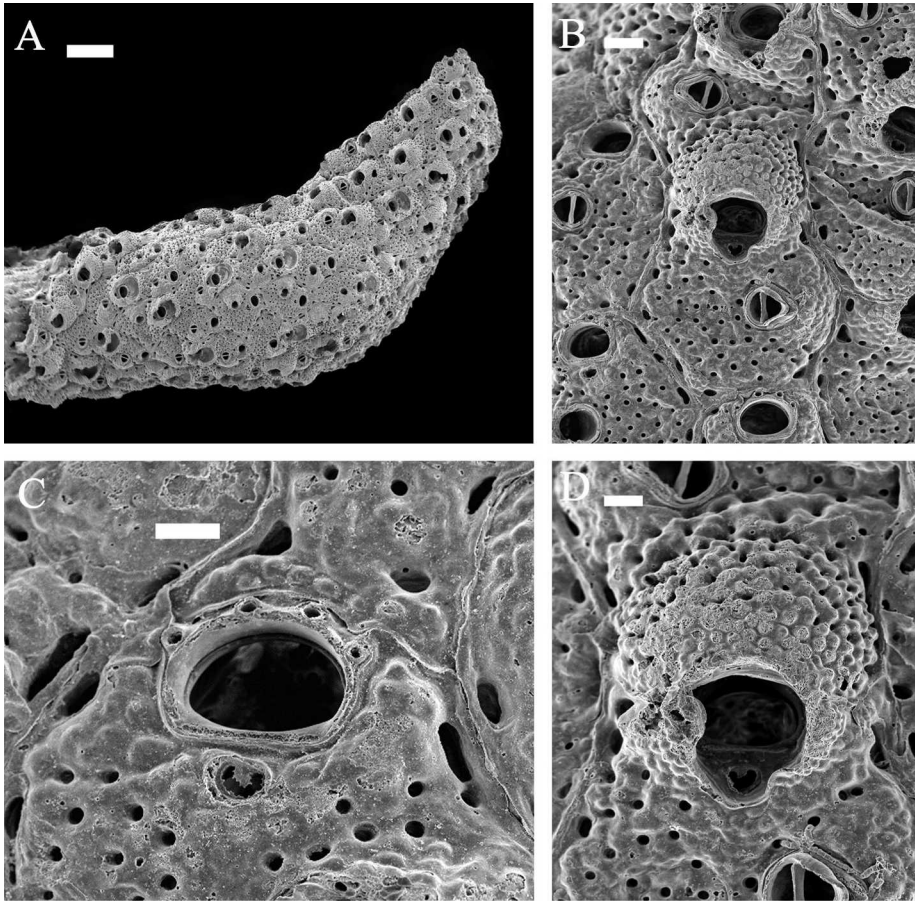
Figure 26. Microporella protea . Hassler Box 12. MCZ 100134. A. Colony encrusting a dead erect bryozoan. Scale bar = 500 \mu\text{m} . B. Group of zooids with ovicelled zooid at center. Scale bar = 100 \mu\text{m} . C. Close-up of orifice and ascopore. Scale bar = 50 \mu\text{m} . D. Close-up of ovicell, showing embedded ascopore. Scale bar = 50 \mu\text{m} .
