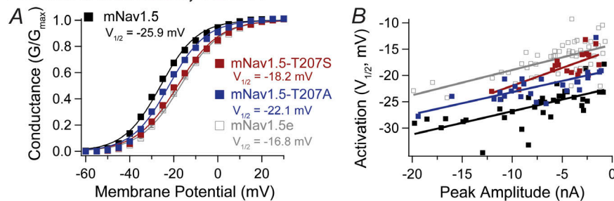
Figure 7. A constrained hydrogen bond donor is required at position 207 to yield the hyperpolarized activation parameters of mNav1.5. (A) Introducing T207A in mNav1.5 results in an activation profile that is also depolarized compared with mNav1.5, suggesting that the rigidity of the residue at this position is critical to the altered gating behavior. The activation V_{1/2} of mNav1.5-T207A (blue) was -22.1 \pm 0.56 mV ( n = 26 ), distinct from mNav1.5 ( P < 0.001 ). Admittedly, though, the shift is not as strong as that of mNav1.5-T207S (red, P < 0.001 ). The slope factor k was 8.3 \pm 0.13 . (B) The y-intercept of the mNav1.5-T207A scatter measured -18.9 \pm 0.16 mV, distinct from both with mNav1.5 ( P < 0.001 ) and mNav1.5-T207S ( P < 0.01 ). The regression line slope was 0.42 \pm 0.02 mV/nA. (C) Substituting S207A in mNav1.5e had virtually no effect, highlighting the importance of losing the sterically constrained threonine residue in causing the shift in channel activation. The activation V_{1/2} of mNav1.5e-S207A (blue) was -16.8 \pm 0.49 mV ( n = 20 ), coinciding with mNav1.5e ( P = 1.00 ). The slope factor k was 9.5 \pm 0.11 . (D) The y-intercept of the mNav1.5e-S207A scatter measured -14.5 \pm 0.14 mV, indistinguishable from mNav1.5e ( P = 0.95 ). The regression line slope was 0.37 \pm 0.02 mV/nA.
