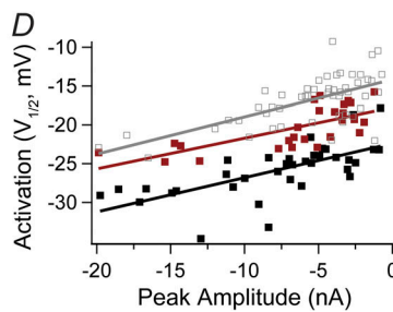
Figure 4. The threonine-serine switch at position 207 also influences channel activation. (A) Introducing T207S into mNav1.5 also causes a shift in the activation profile toward that of mNav1.5e. The activation V_{1/2} of mNav1.5-T207S (red) was -18.2 \pm 0.64 mV ( n = 17 ), distinct from mNav1.5 ( P < 0.001 ) and apparently overlapping with mNav1.5e ( P = 0.30 ). The slope factor k was 9.3 \pm 0.15 . (B) The y-intercept of the mNav1.5-T207S scatter measured -15.2 \pm 0.21 mV, falling between mNav1.5 ( P < 0.001 ) and mNav1.5e ( P < 0.05 ). The regression line slope was steeper than usual, at 0.68 \pm 0.04 mV/nA. (C) Replacing S207T in mNav1.5e produces an intermediate phenotype in terms of channel activation. The activation V_{1/2} of mNav1.5e-S207T (red) was -20.3 \pm 0.53 mV ( n = 26 ), distinct from both mNav1.5e ( P < 0.001 ) and mNav1.5 ( P < 0.001 ). The slope factor k was 9.6 \pm 0.14 . (D) The y-intercept of the mNav1.5e-S207T scatter measured -17.7 \pm 0.13 mV, different from both mNav1.5 ( P < 0.001 ) and mNav1.5e ( P < 0.001 ). The regression line slope was 0.40 \pm 0.02 mV/nA.
