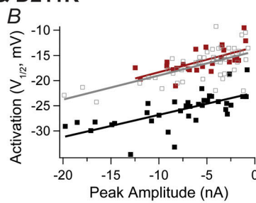
Figure 5. Combined, the Thr/Ser and Asp/Lys switches account for the full gating difference between mNav1.5 and mNav1.5e. (A) Introducing both T207S and D211K into mNav1.5 results in an activation profile that is indistinguishable from that of mNav1.5e. The activation V_{1/2} of mNav1.5-T207S-D211K (red) was -16.2 \pm 0.50 mV ( n = 25 ), overlapping with mNav1.5e ( P = 0.64 ) yet distinct from mNav1.5 ( P < 0.001 ). The slope factor k was 9.3 \pm 0.10 . (B) The y-intercept of the mNav1.5-T207S-D211K scatter measured -13.3 \pm 0.16 mV, coinciding with mNav1.5e ( P = 0.43 ) but remaining distinct from mNav1.5 ( P < 0.001 ). The regression line slope was 0.50 \pm 0.02 mV/nA. (C) Replacing both S207T and K211D in mNav1.5e produces a phenotype similar to that of mNav1.5. The activation V_{1/2} of mNav1.5e-S207T-K211D (red) was -27.6 \pm 0.51 mV ( n = 24 ), distinct from mNav1.5e ( P < 0.001 ) yet identical to mNav1.5 ( P = 0.10 ). The slope factor k was 8.8 \pm 0.16 . (D) The y-intercept of the mNav1.5e-S207T-K211D scatter measured -23.9 \pm 0.17 mV, overshooting mNav1.5 in the negative direction ( P < 0.05 ) yet still very distinct from mNav1.5e ( P < 0.001 ). The regression line slope was 0.46 \pm 0.02 mV/nA.
