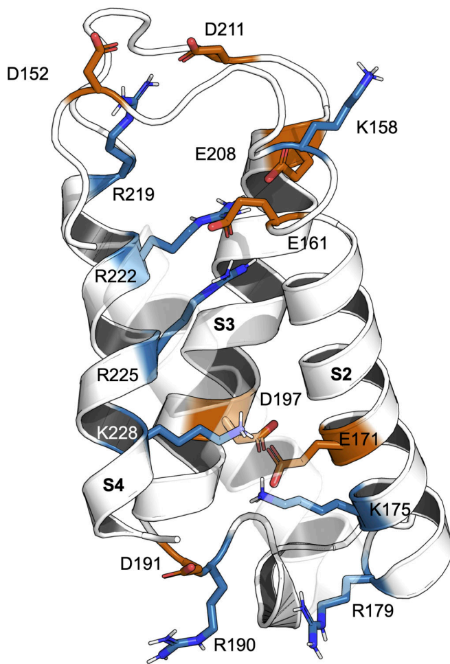
Figure 9. Overview of key charged residues present within the VSD. The VSD of DI in mNav1.5. The VSD (white) contains four transmembrane helices (S1–S4, labeled in bold) with a number of positively (blue) and negatively (orange) charged residues that make up critical salt bridges during S4 translocation during mNav1.5 depolarization. Note that the S1 label has been removed and the helix shown as transparent for clarity.
