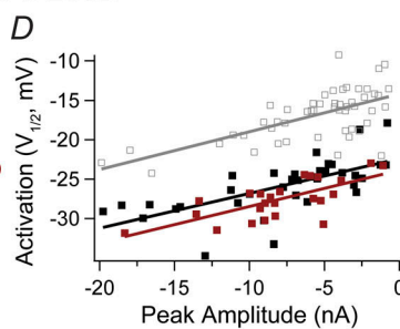
Figure 5. Combined, the Thr/Ser and Asp/Lys switches account for the full gating difference between mNav1.5 and mNav1.5e. (A) Introducing both T207S and D211K into mNav1.5 results in an activation profile that is indistinguishable from that of mNav1.5e. The activation V_{1/2} of mNav1.5-T207S-D211K (red) was -16.2 \pm 0.50 mV ( n = 25 ), overlapping with mNav1.5e ( P = 0.64 ) yet distinct from mNav1.5 ( P < 0.001 ). The slope factor k was 9.3 \pm 0.10 . (B) The y-intercept of the mNav1.5-T207S-D211K scatter measured -13.3 \pm 0.16 mV, coinciding with mNav1.5e ( P = 0.43 ) but remaining distinct from mNav1.5 ( P < 0.001 ). The regression line slope was 0.50 \pm 0.02 mV/nA. (C) Replacing both S207T and K211D in mNav1.5e produces a phenotype similar to that of mNav1.5. The activation V_{1/2} of mNav1.5e-S207T-K211D (red) was -27.6 \pm 0.51 mV ( n = 24 ), distinct from mNav1.5e ( P < 0.001 ) yet identical to mNav1.5 ( P = 0.10 ). The slope factor k was 8.8 \pm 0.16 . (D) The y-intercept of the mNav1.5e-S207T-K211D scatter measured -23.9 \pm 0.17 mV, overshooting mNav1.5 in the negative direction ( P < 0.05 ) yet still very distinct from mNav1.5e ( P < 0.001 ). The regression line slope was 0.46 \pm 0.02 mV/nA.
