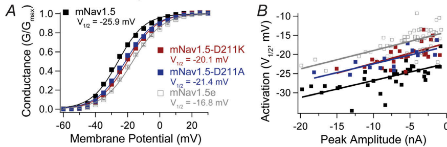
Figure 6. The presence of a negative charge at position 211 is essential to the hyperpolarized gating profile of mNav1.5. (A) Introducing D211A in mNav1.5 results in an activation profile that is indistinguishable from the mutant mNav1.5-D211K, as if loss of the negative charge were more critical to the altered gating shift than gaining the positive charge. The activation V_{1/2} of mNav1.5-D211A (blue) was -21.4 \pm 0.75 mV ( n = 14 ), similar to mNav1.5-D211K (red, P = 0.64 ). The slope factor k was 8.8 \pm 0.19 . (B) The y-intercept of the mNav1.5-D211A scatter measured -17.9 \pm 0.07 mV, coinciding with mNav1.5-D211K ( P = 0.92 ). The regression line slope was 0.46 \pm 0.01 mV/nA. (C) Substituting K211A in mNav1.5e also produces a small but nonnegligible shift, taking on a phenotype between mNav1.5e-K211D and mNav1.5e, suggesting that the presence of the positive charge may matter to a limited degree. The activation V_{1/2} of mNav1.5e-K211A (blue) was -19.8 \pm 0.50 mV ( n = 42 ), distinct from both mNav1.5e-K211D (red, P < 0.001 ) and mNav1.5e ( P < 0.001 ). The slope factor k was 8.5 \pm 0.18 . (D) The y-intercept of the mNav1.5e-K211A scatter measured -15.7 \pm 0.07 mV, distinct from both mNav1.5e-K211D ( P < 0.001 ) and mNav1.5e ( P < 0.05 ). The regression line slope was 0.47 \pm 0.01 mV/nA.
