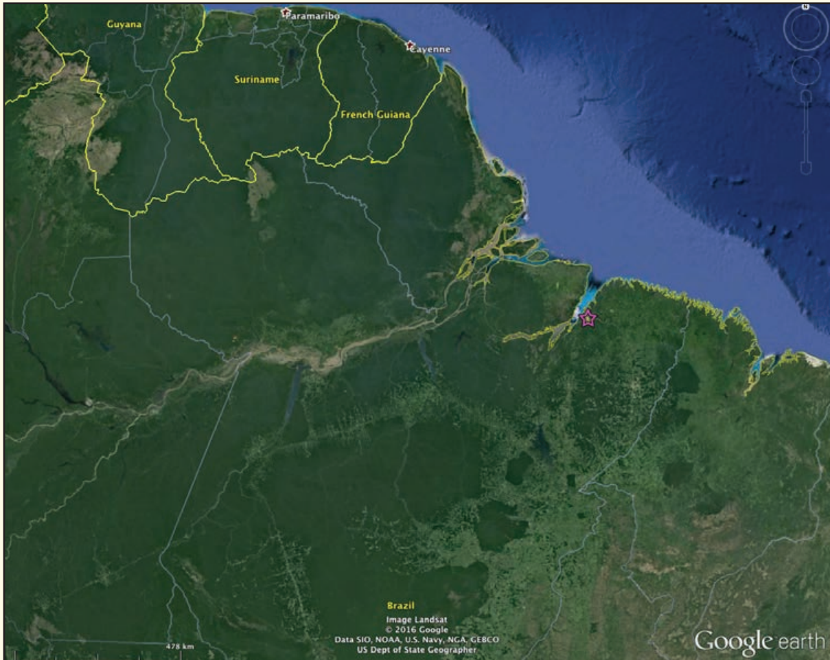
Map. 13. Distribution of Epictia albifrons in northeastern Brazil.
