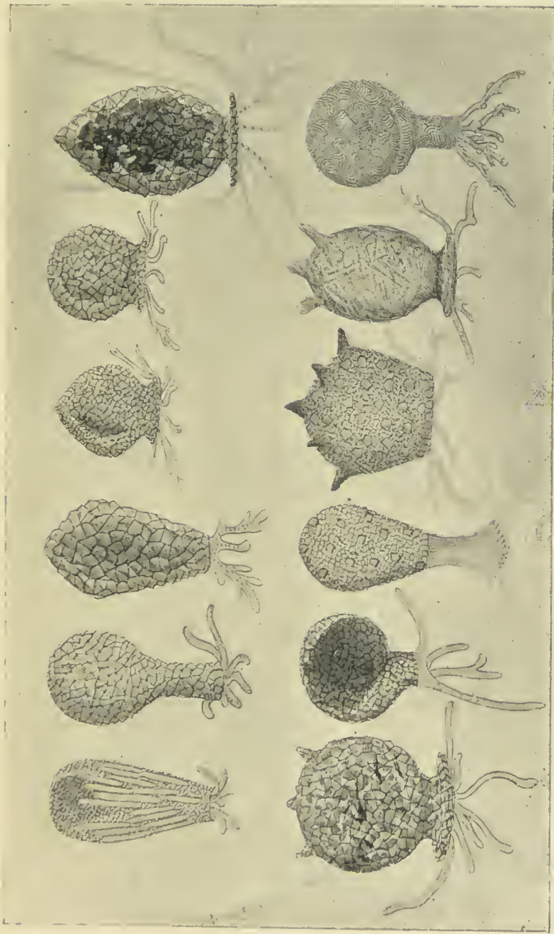
Fig. 40. — Diffugia , Fresh-water Rhizopods (after Leidy). Ranging from the \frac{1}{100} th to the \frac{1}{20} th of an inch in diameter.
