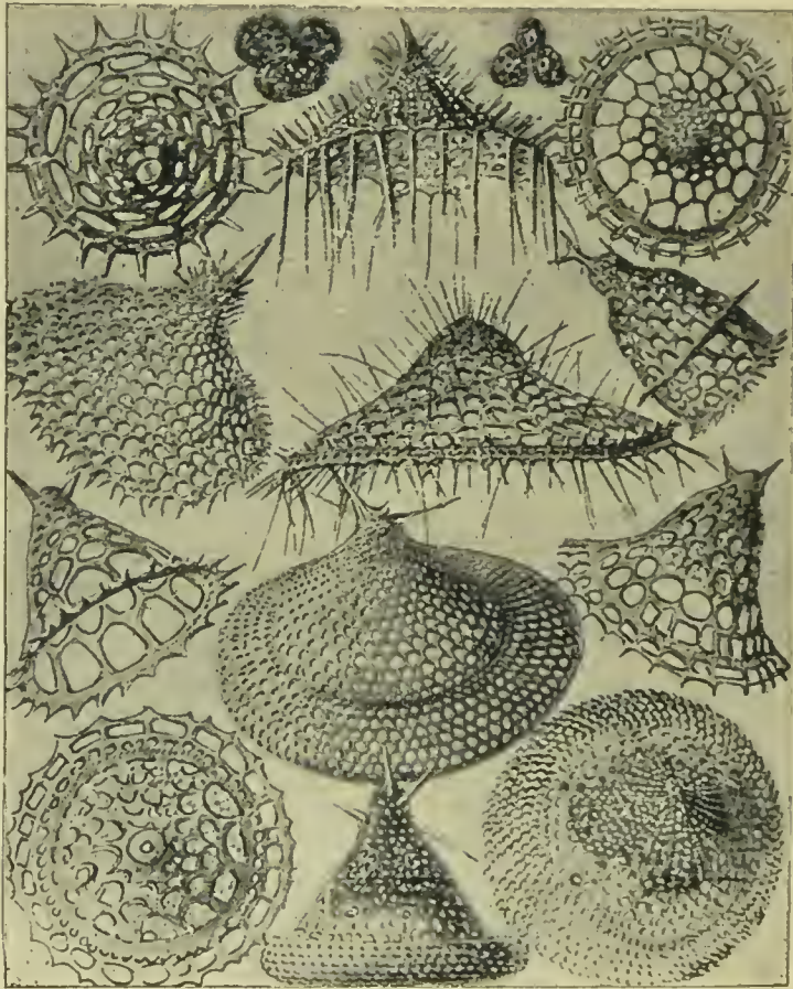
Fig. 22.—Radiolaria. (Challenger_Series.)
