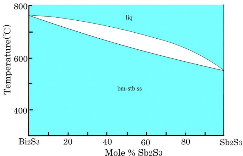
Figure 2. Phase relations of the Bi 2 S 3 -Sb 2 S 3 join in the Bi-Sb-S system.
