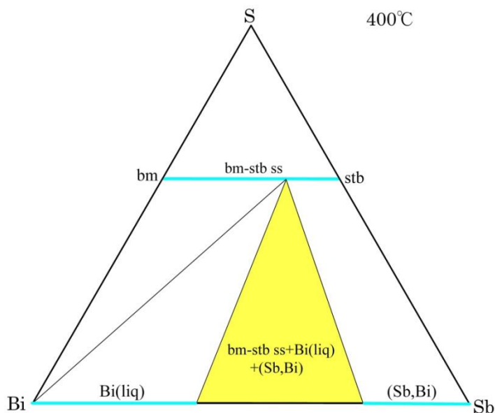
Figure 3. Phase diagram of the Bi-Sb-S system at 400°C.
