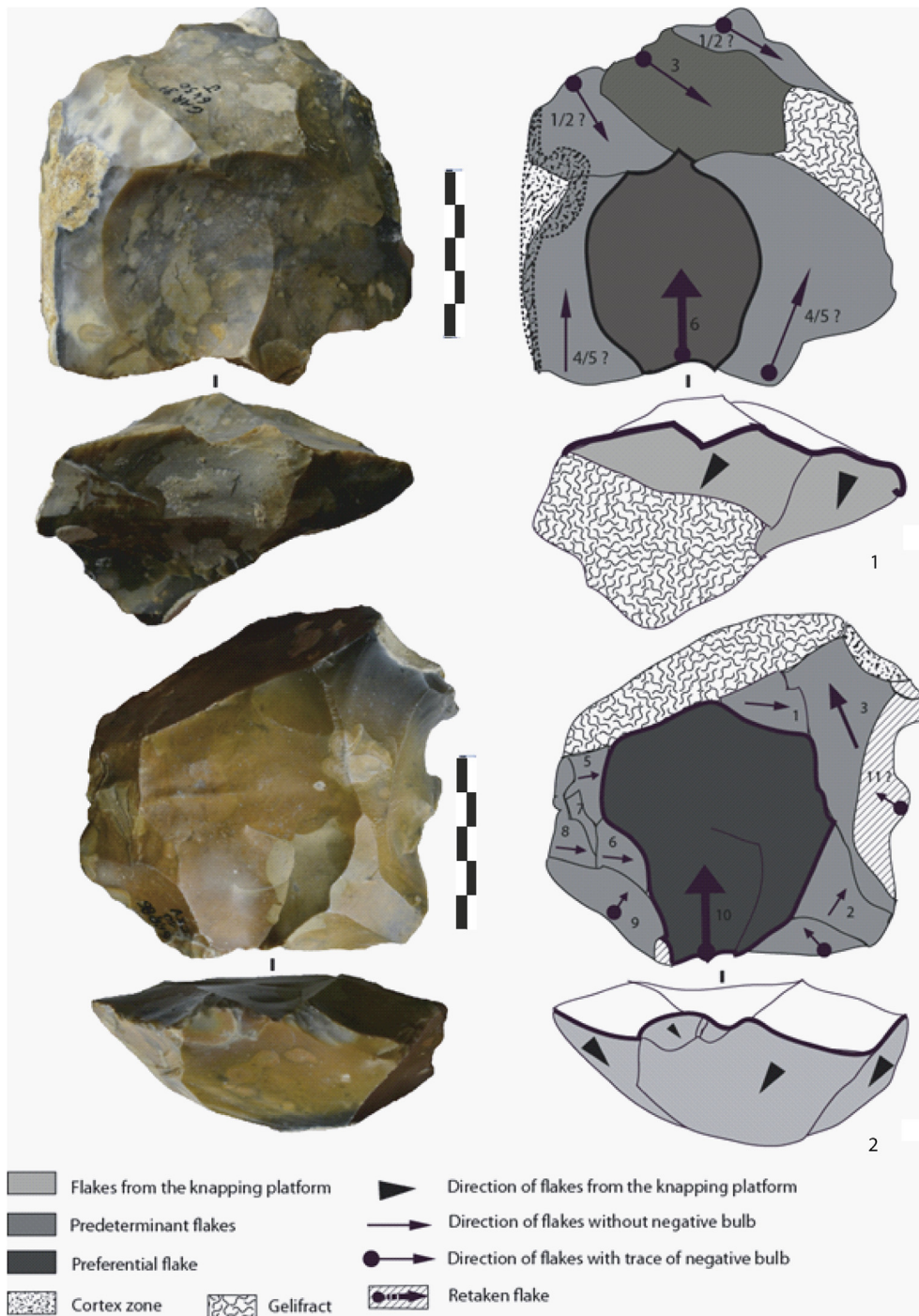
Figure 4. A) Cagny-La-Garenne II—Level J (beginning of the alluvial sequence). B) Cagny-la-Garenne I—Level CXV (final alluvial sequence). Both preferential Levallois cores. Drawings and pictures: A. Lamotte.
