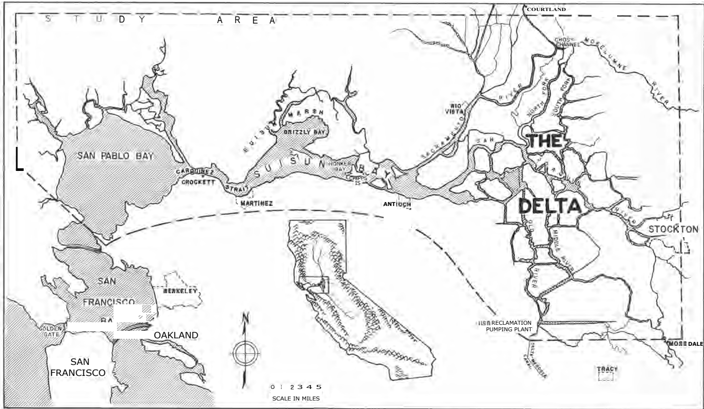
FIGURE 1. Map of the Sacramento-San Joaquin Estuary.
