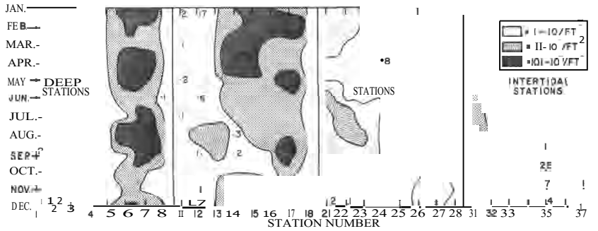
FIGURE 14. Average numbers of Sirebaspia benedicti per square foot sample each month at four depths along eight transects in the study area.
