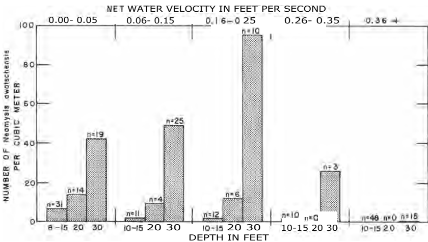
FIGURE 3. Neomysis awatzensis per cubic meter in relation to net water velocity and depth, Sacramento-San Joaquin Delta. Number above figure is sample size.
