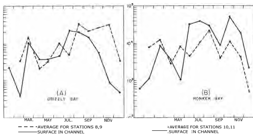
FIGURE 13. Monthly concentrations of total net zooplankton from the shallow flats of Grizzly and Honker Bays and from a nearby surface channel station. The broken lines connect the monthly means of two "flats" stations. Solid lines connect the monthly concentration at the nearest surface channel station.
