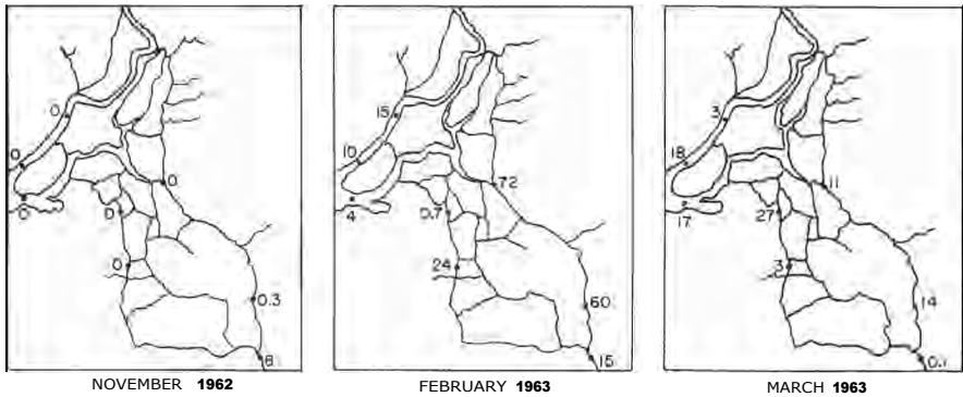
FIGURE 11. Late fall and winter collection of young (less than 5 mm) Corbicula fluminea . Numbers on the maps are the mean number of C. fluminea collected during the month.
