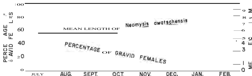
FIGURE 4. Mean length of Neomysis awatschensis and percentage of gravid females in Sacramento-San Joaquin Delta, July 1963 to February 1964.
