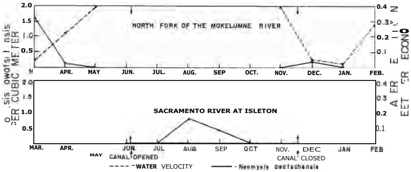
FIGURE 2. Neomysis awatzensis per cubic meter and the net water velocity in the Sacramento River at Isleton and the North Fork of the Mokelumne River, March 1963 to February 1964.
