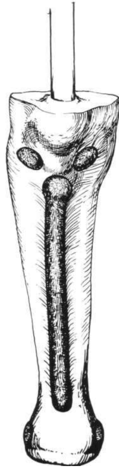
Fig. 32. Model with skived leather patches applied to provide in finished socket relief for sensitive areas.
