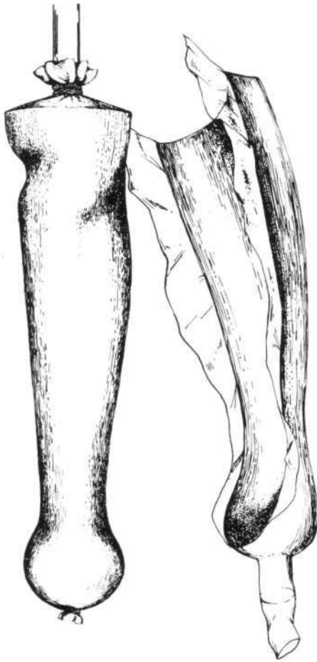
Fig. 35. Removal of laminate to be used later in fabrication of cover for opening in socket.
