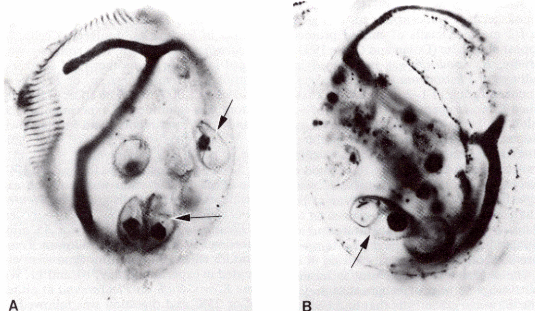
Fig. 1. Examples of protargol-stained specimens of Euplotes woodruffi showing the remains (arrows) of ingested Pleuronema : a cell from a log growth phase culture (A), and a cell collected on 5 August 1986 from station 845 in Chesapeake Bay (B).
