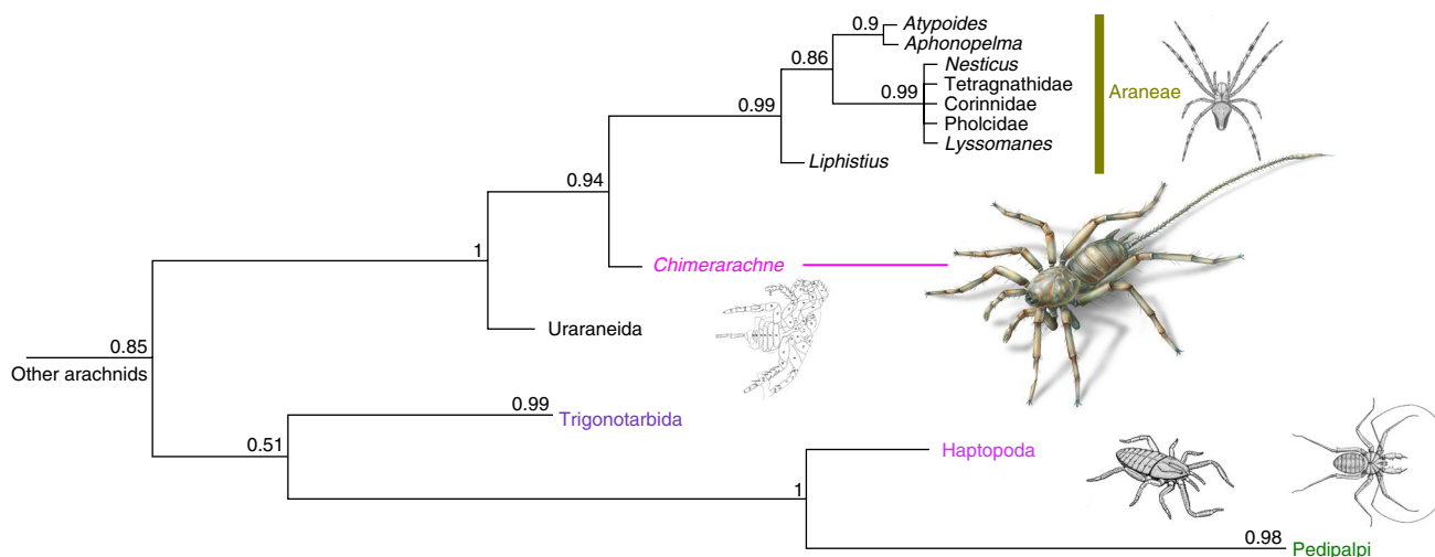
Fig. 5 | Phylogenetic relationships. Consensus cladogram (Bayesian majority rule consensus with support values) showing the position of C. yingi within the Pantetrapulmonata branch of the arachnids, which encompasses the spiders and their closest relatives (see Supplementary Fig. 3 for the full annotated tree). Both Attercopus and Permarachne are incomplete and scoring them individually collapses the tree, thus we combined characters from the two genera into one terminal Uraraneida. Full methods, results, discussion and sources for the line drawings are provided in the Supplementary Information.
