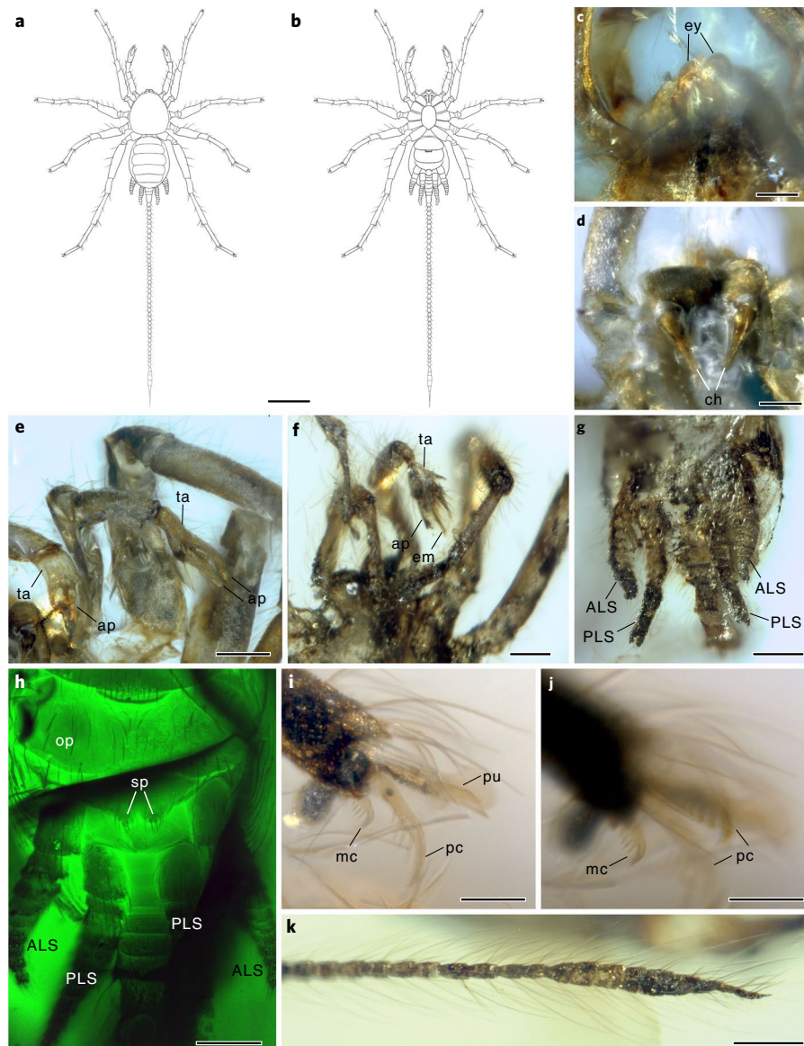
Fig. 3 | Morphological details and reconstruction. a, b , Reconstruction in dorsal ( a ) and ventral view ( b ). c , Eyes in NIGP166870. d , Chelicerae in NIGP166870. e , Ventral palps in NIGP166870. f , Ventral palps in NIGP166871. g , Spinnerets in NIGP166871. h , Confocal laser scanning microscope image of the abdomen in NIGP166870. i, j , Leg II claw in NIGP166870. k , Flagellum in NIGP166871. ap, apophysis; ALS, anterior lateral spinneret; ch, chelicera; em, embolus; ey, eye; mc, median claw; op, operculum; pc, paired claws; PLS, posterior lateral spinneret; pu, pulvillus; sp, spigots; ta, tarsus. Scale bars: 1 mm in a and b ; 0.2 mm in e–h and k ; 0.1 mm in c and d ; 0.05 mm in i and j .
