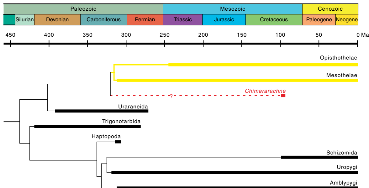
Fig. 6 | Evolutionary history of spiders and spider-related arachnids. Thick lines indicate the known extent of the fossil record. Branches representing modern spiders are yellow. The branch of Chimerarachne is red. See Supplementary Information for details of the phylogenetic analysis.
