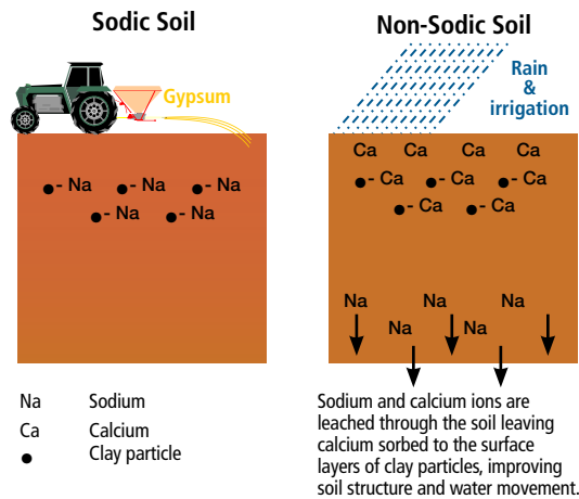
Figure 12 Correction of sodic soil. Source: (Kelly & Renagasamy 2006)
