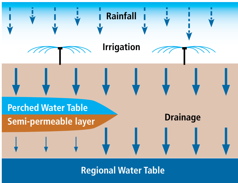
Figure 15 Formation of perched water table.
