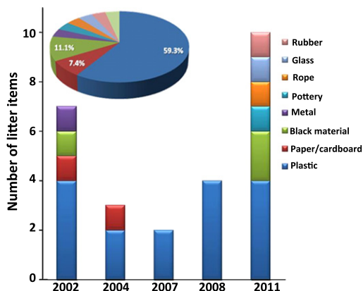
Fig. 3. Types of litter recorded from seafloor photographs taken between 2002 and 2011.
