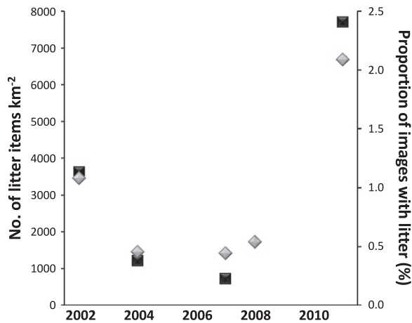
Fig. 2. Abundance of litter items at HAUSGARTEN central station (2500 m depth) between 2002 and 2011. Black symbols represent mean litter densities (number km -2 ); grey symbols represent the proportion of images showing litter every year.
