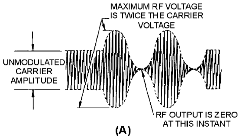
Figure 1-1A. Conditions for 100-percent modulation.
