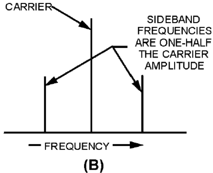
Figure 1-1B. Conditions for 100-percent modulation.
