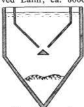
Emscher-brønd.
