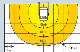
Max. illuminance 1600 lx at a distance of 40 cm (switching stage II)
