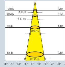
DECOSTAR® TITAN 46865 VWFL
