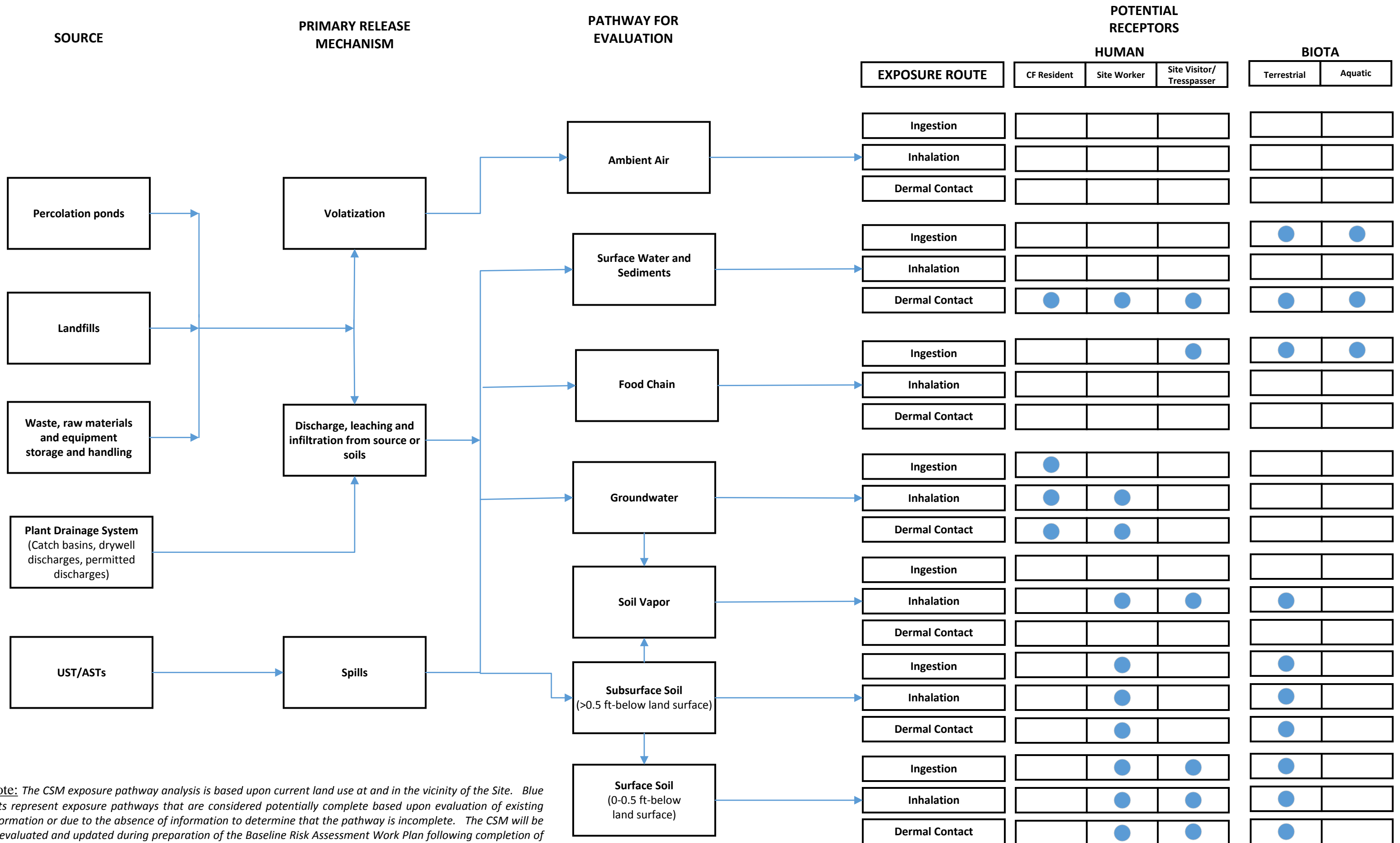
Figure 10. Preliminary Conceptual Site Model Columbia Falls Aluminum Company, MT
