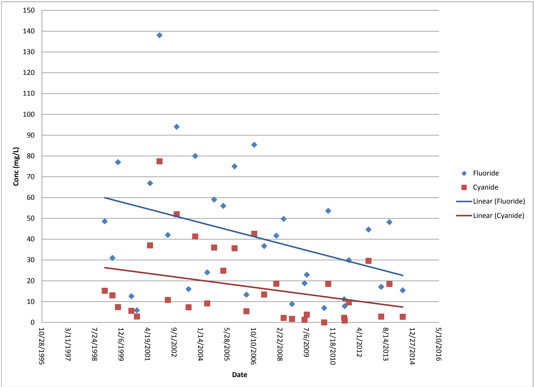
Figure 7. Historical Cyanide and Fluoride Concentrations in MPDES Groundwater Sampling Location W-11 Columbia Falls Aluminum Company, Columbia Falls, Montana
