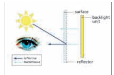
Transflective Panel
