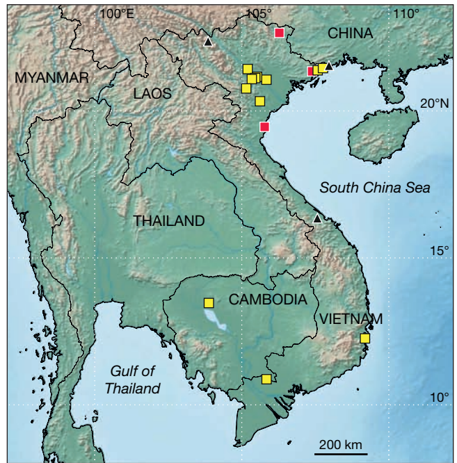
FIG. 28. — Distribution of Syzygium imitans Merr. & L.M.Perry (▲), Syzygium jambos (L.) Alston (■) and Syzygium levinei (Merr.) Merr. & L.M.Perry (■) in Indochina.
