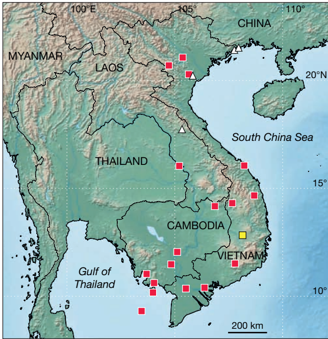
FIG. 12. — Distribution of Syzygium championii (Benth.) Merr. & L.M.Perry (Δ), Syzygium chantaranothaianum W.K.Soh & J.Parn. (■) and Syzygium claviflorum (Roxb.) Wall. ex Steudel (■) in Indochina.
