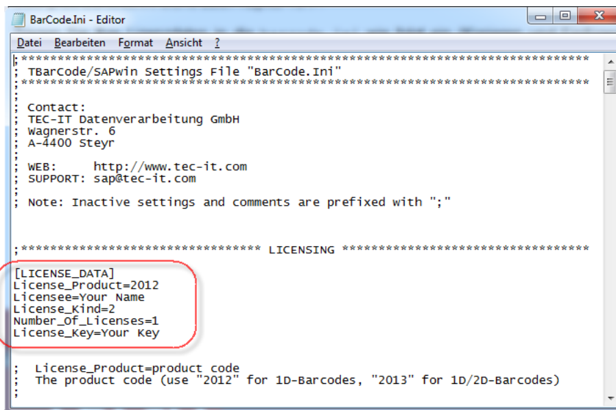
Figure 37: Barcode.ini
