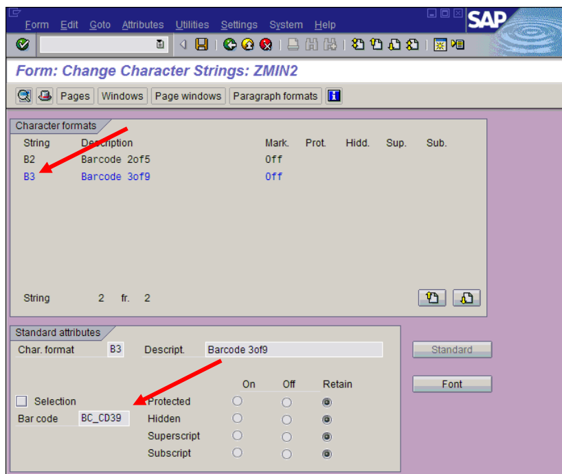
Figure 15: Character Format Definition in a SAPscript form
