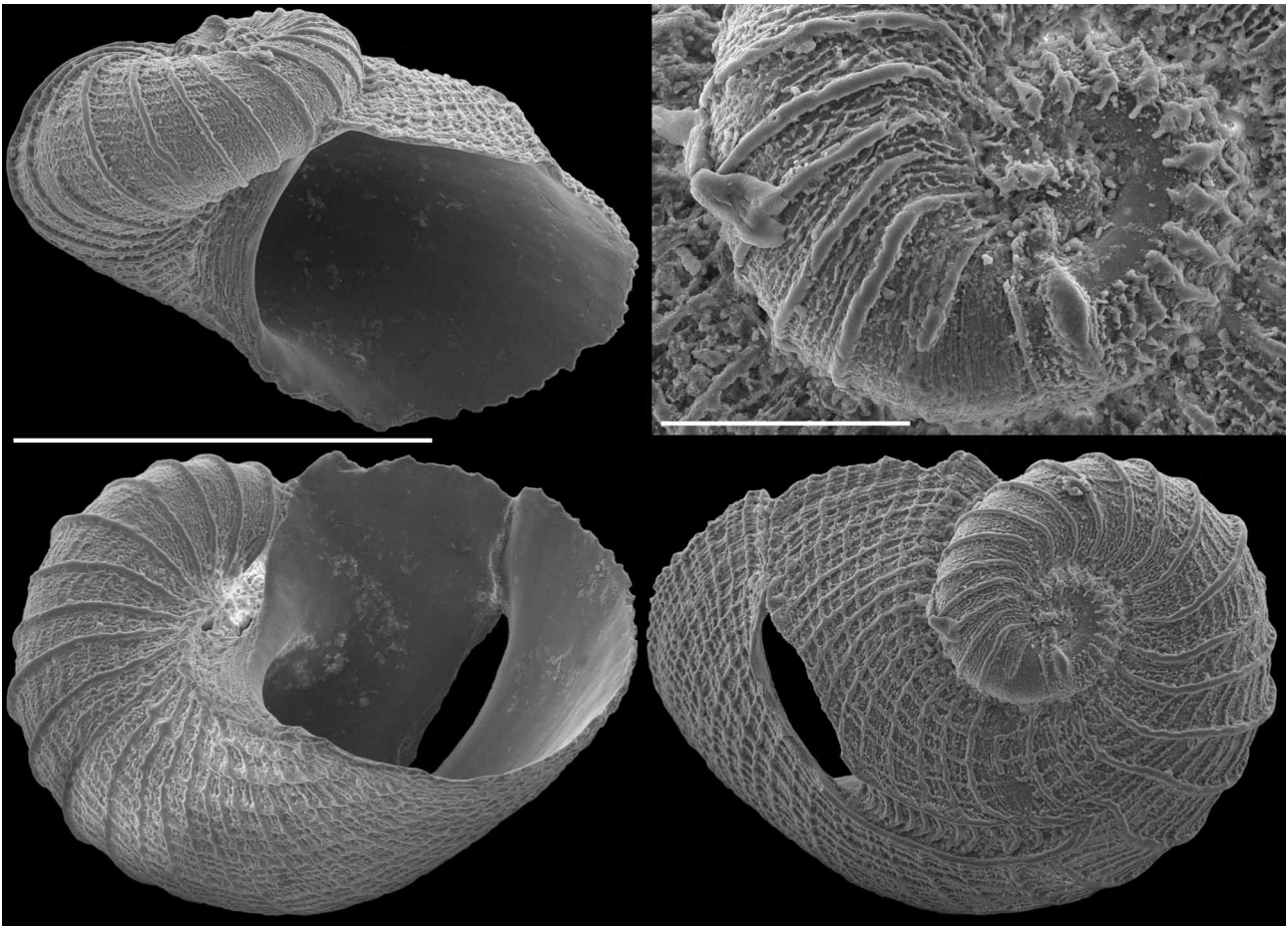
FIGURE 4. Holotype of Sinezona milleri n. sp. SBMNH 83548. North side, Ikei Jima, Okinawa, Japan. Scale bar shell = 500 \mu m. Scale bar protoconch = 100 \mu m.
