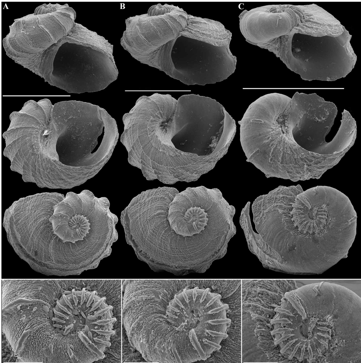
FIGURE 2. Paratypes of Sinezona costulata n. sp. A–C. SBMNH 83545. Peninsula towards shrine, Cape Manazuru, Kanagawa Prefecture, Japan. Scale bars shell = 500 µm. Scale bars protoconch = 100 µm.
