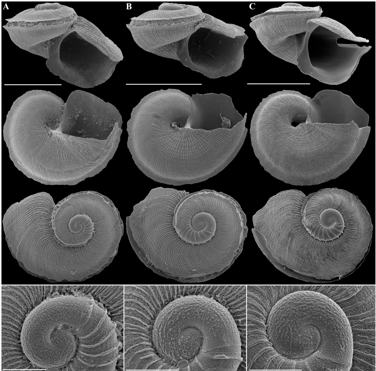
FIGURE 9. Paratypes of Anatoma parageia n. sp. A.–B. SBMNH 83553. C. UMUT RM29235. Peninsula towards shrine, Cape Manazuru, Kanagawa Prefecture, Japan. Scale bars shell = 500 \mu m. Scale bars protoconch = 100 \mu m.
