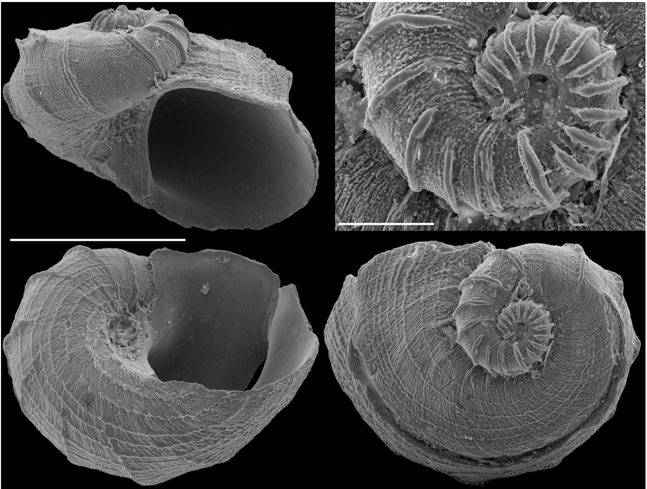
FIGURE 1. Holotype of Sinezona costulata n. sp. SBMNH 83544. Peninsula towards shrine, Cape Manazuru, Kanagawa Prefecture, Japan. Scale bar shell = 500 \mu m. Scale bar protoconch = 100 \mu m.
