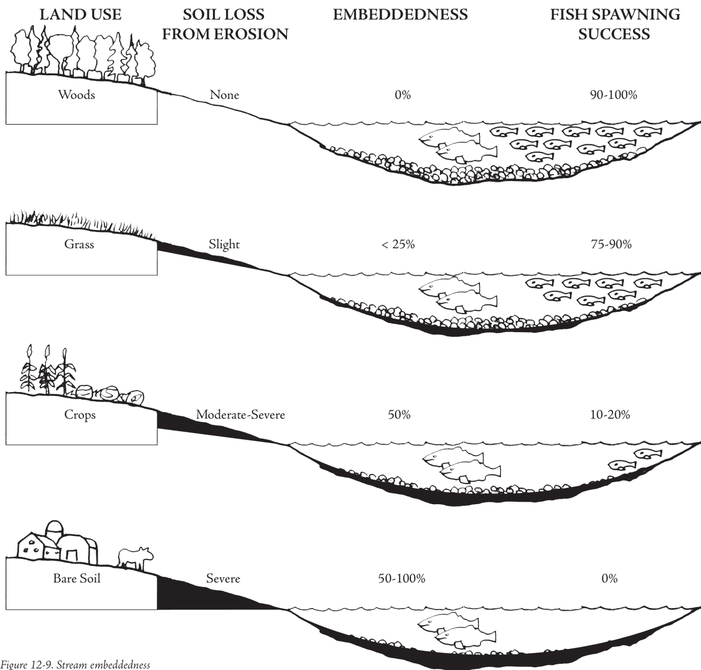
Figure 12-9. Stream embeddedness
