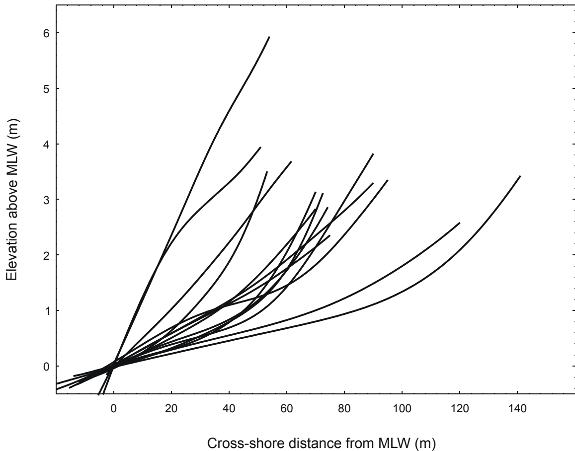
Fig. 4.2 - Overview of beach profiles from beaches studied during this thesis (MLW = Mean Low water)
