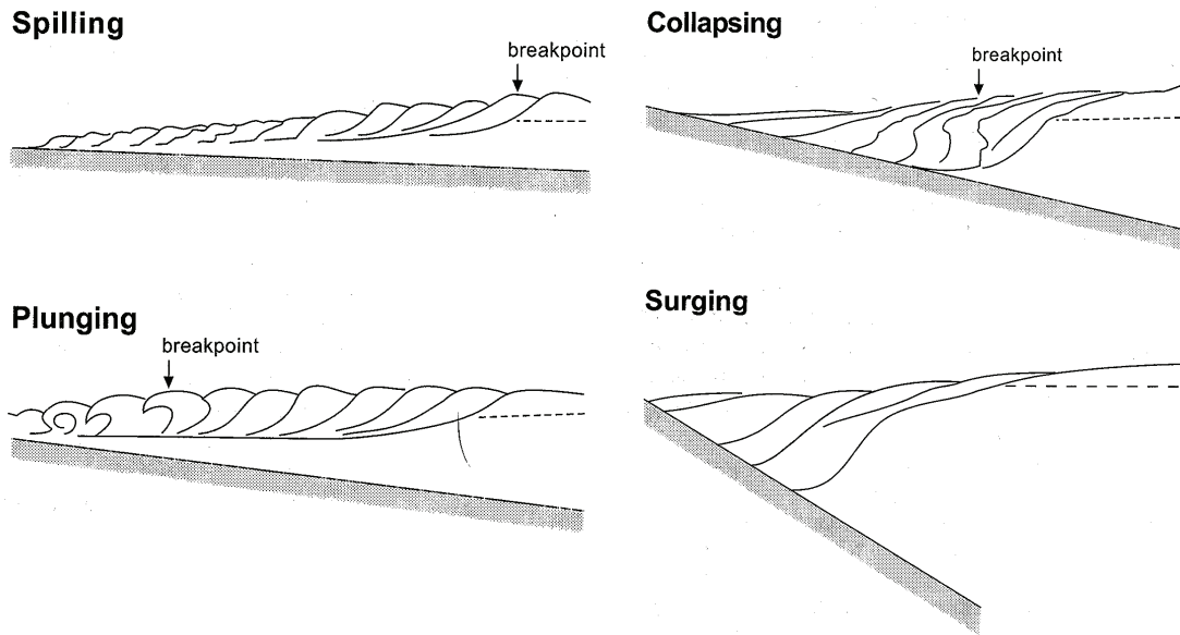
Fig. 1.2 - Types of breakers (modified from Short, 1999).
