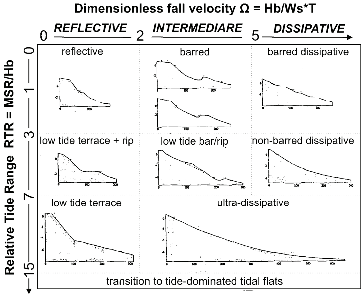
Fig. 1.3 - Beach classification scheme from Masselink and Short (1993).
