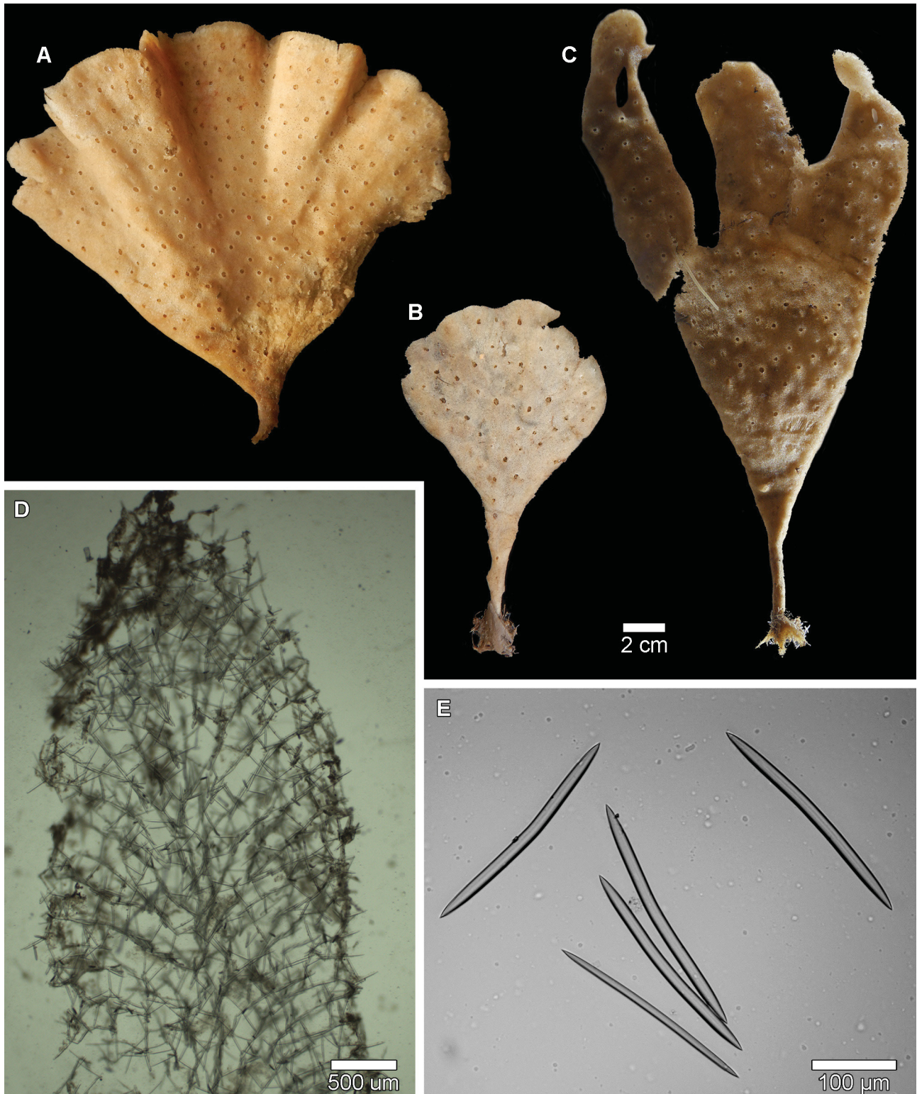
FIGURE 3. Cladocroce spatula (Lundbeck, 1902). A–C, collected specimens; D. skeleton showing anisotropic reticulation and axial fibres; E. spicules. Thin oxeas are uncommon and may represent a developmental form.
