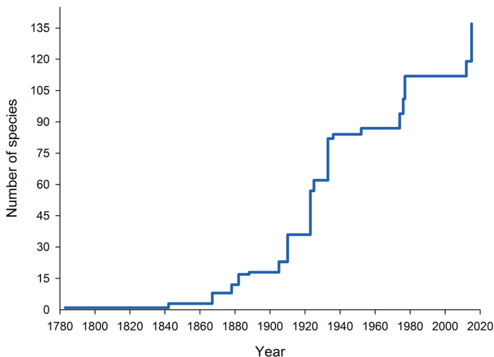
Fig. 1. Increase in the number of Ophiuroidea species reported for South Africa from 1783 to present (137).
