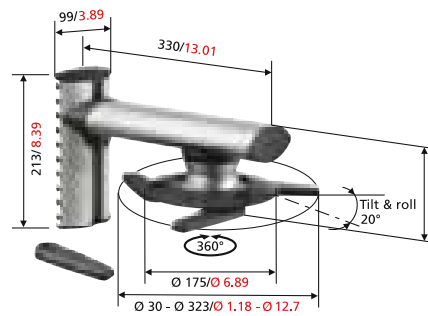
Complete projector wall solution (EPW 6560 and EPA 6505)
