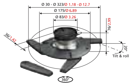
Complete projector ceiling solution (EPC 6540 and EPA 6505)
