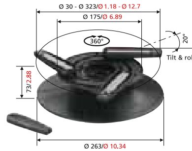
Complete projector table solution (EPT 6520 and EPA 6505)
