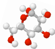
Glucose Molecule
