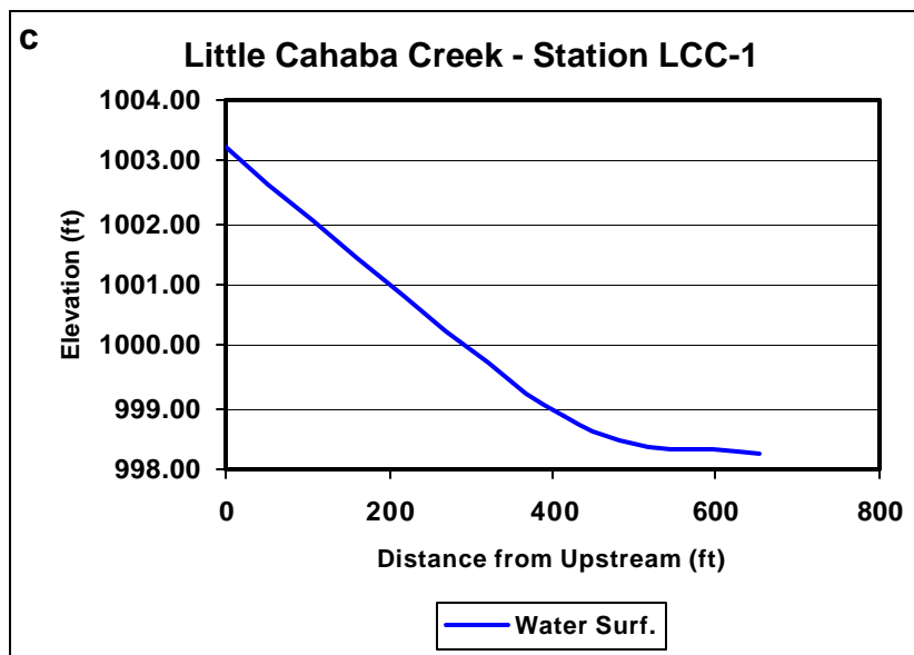
Figure 7. Hydraulic geometry at Little Cahaba Creek Station LCC-1, located at Camp Coleman Road Bridge; Latitude: 33° 37' 34"; Longitude: 86° 33' 58": a. cross-section; b. planform; and c. longitudinal water-surface profile; water surface slope = 0.81%; Surveyed on 09/11/02.
