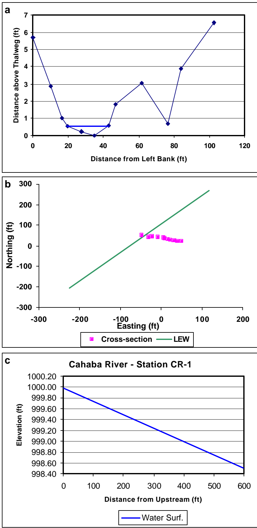
Figure 1. Hydraulic geometry at CahabaRiver Station CR-1, located at Happy Hollow Rd. near CR 132; Latitude: 33/ 38' 39"; Longitude: 86/35' 45": a. cross-section; b.planform; and c. longitudinal water-surface profile; water surface slope = 0.25%; Surveyed on 09/11/02.
