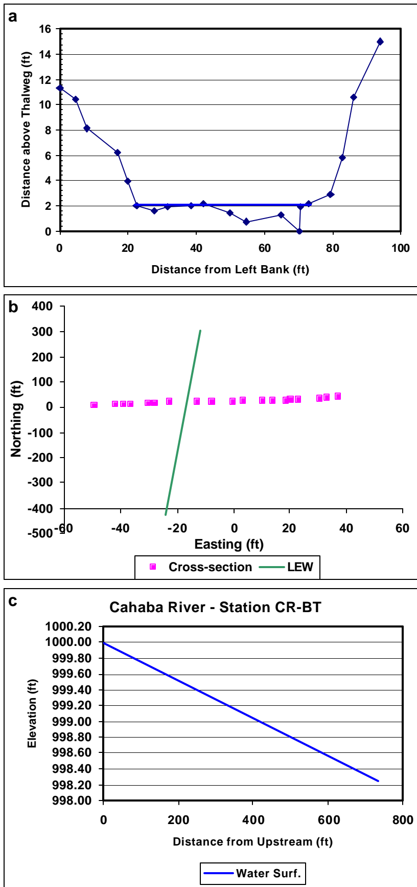
Figure 10. Hydraulic geometry at Cahaba River Station CR-BT, located at CR 10 below Trussville WWTP; Latitude: 33/36' 16.5"; Longitude: 86/32' 56.5"; a. cross-section ; b. planform; and c. longitudinal water-surface profile; water surface slope = 0.24%; Surveyed on 09/11/02.
