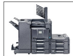
Standard Printer + *MT-730(B) 7 bins Mailbox Sorter + *AK-736 Mailbox Attachment Kit + *DF-790(B) 4,000 sheet Finisher + *AK-735 Bridge Unit for Finisher + *PF-740 Paper Feeder x 2 + *PF-780 Multimedia Tray and Paper Pass Unit + *BF-730 Booklet & Tri-Folding Unit
