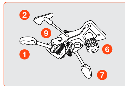
R1 Rocking Tilt
