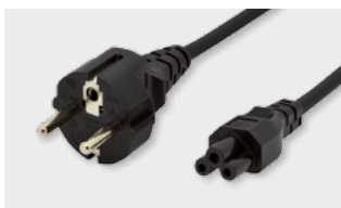
CEE 7/7-C5, M/F, H5VV-F3G
