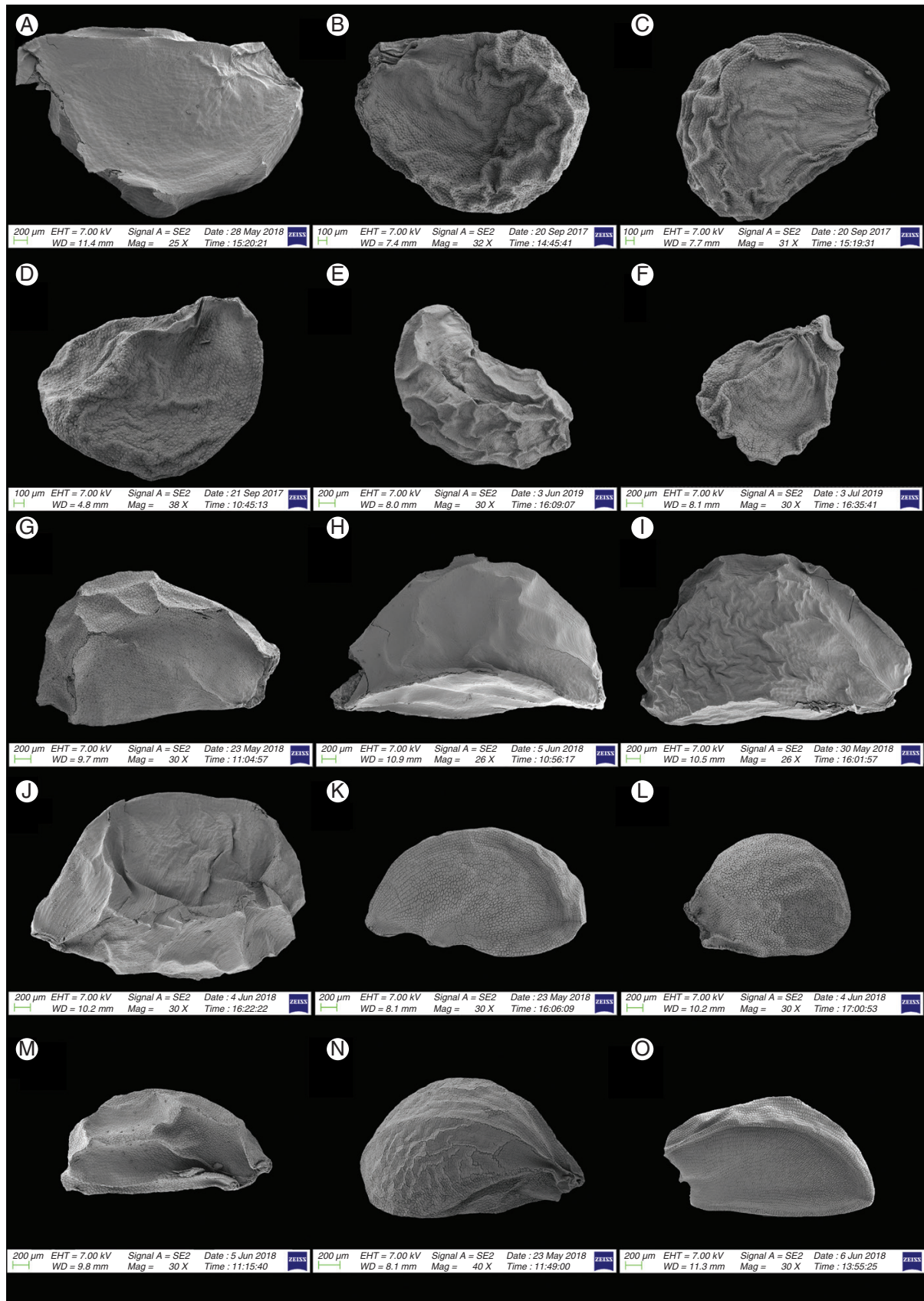
FIG. 3. SEM micrographs of seeds of 15 Allium species. (A–F) Subg. Melanocrommyum : (A) A. regelii (sect. Regeloprason ); (B) A. cupuliferum (sect. Regeloprason ); (C) A. isakulii (sect. Regeloprason ); (D) A. taeniopetalum (sect. Stellata ); (E) A. cardiostemon (sect. Melanocrommyum ); (F) A. woronowii (sect. Melanocrommyum ). (G–K) Subg. Butomissa : (G) A. oreoprasum (sect. Austromontana ); (H) A. ramosum (sect. Butomissa ); (I) A. ramosum (sect. Butomissa ); (J) A. tuberosum (sect. Butomissa ); (K) A. aff. tuberosum . (L, M) Subg. Cyathophora : (L) A. mairei (sect. Coleoblastus ); (M) A. cyathophorum (sect. Cyathophora ). (N, O) Subg. Rhizirideum : (N) A. subangulatum (sect. Rhizomatosa ); (O) A. przewalskianum (sect. Eduardia ).
