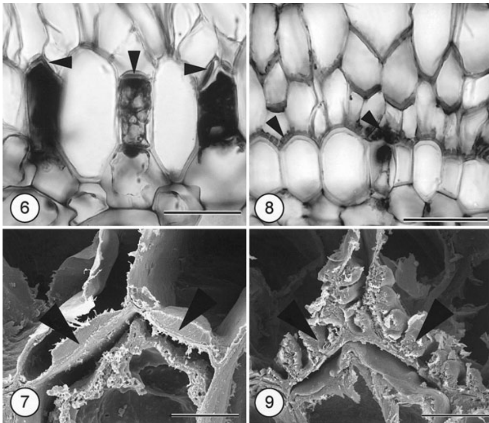
Figures 6–9. Root TS showing endovelum thickenings (arrowheads). Figs 6, 7. Angraecum eburneum . Fig. 6. Light micrograph. Scale bar = 50 \mu\text{m} . Fig. 7. Scanning electron micrograph. Scale bar = 12 \mu\text{m} . Figs 8, 9. Jumellea arachnantha . Fig. 8. Light micrograph. Scale bar = 50 \mu\text{m} . Fig. 9. Scanning electron micrograph. Scale bar = 8.75 \mu\text{m} .
