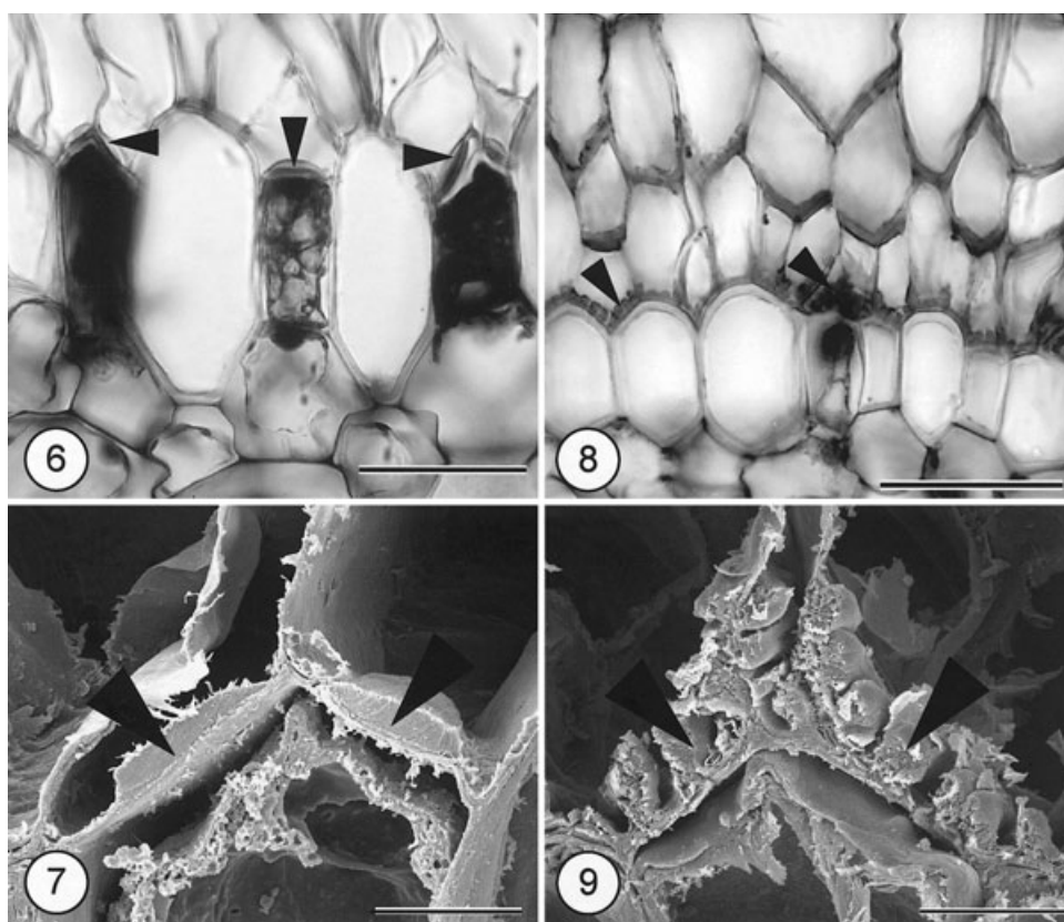
Figures 6–9. Root TS showing endovelamen thickenings (arrowheads). Figs 6, 7. Angraecum eburneum . Fig. 6. Light micrograph. Scale bar = 50 \mu m. Fig. 7. Scanning electron micrograph. Scale bar = 12 \mu m. Figs 8, 9. Jumellea arachnantha . Fig. 8. Light micrograph. Scale bar = 50 \mu m. Fig. 9. Scanning electron micrograph. Scale bar = 8.75 \mu m.
