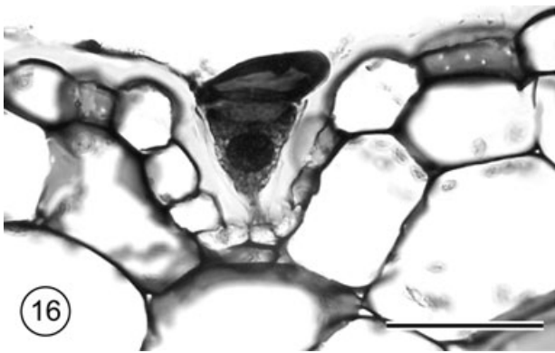
Figure 16. Leaf TS of Angraecum multinominatum showing multicellular, glandular hair within epidermal crypt. Scale bar = 50 \mu\text{m} .
