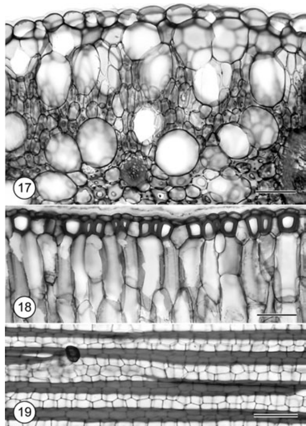
Figures 17–19. Hypodermal cells in leaf. Scale bars = 100 \mu\text{m} . Fig. 17. TS showing hypodermis composed of water-storage cells in Angraecum conchiferum . Fig. 18. TS showing hypodermis composed of thick-walled fibres in Jumellea filicornoides . Fig. 19. Scraping of Tridactyle tridactylites showing elongate fibres of thick-walled hypodermis.
