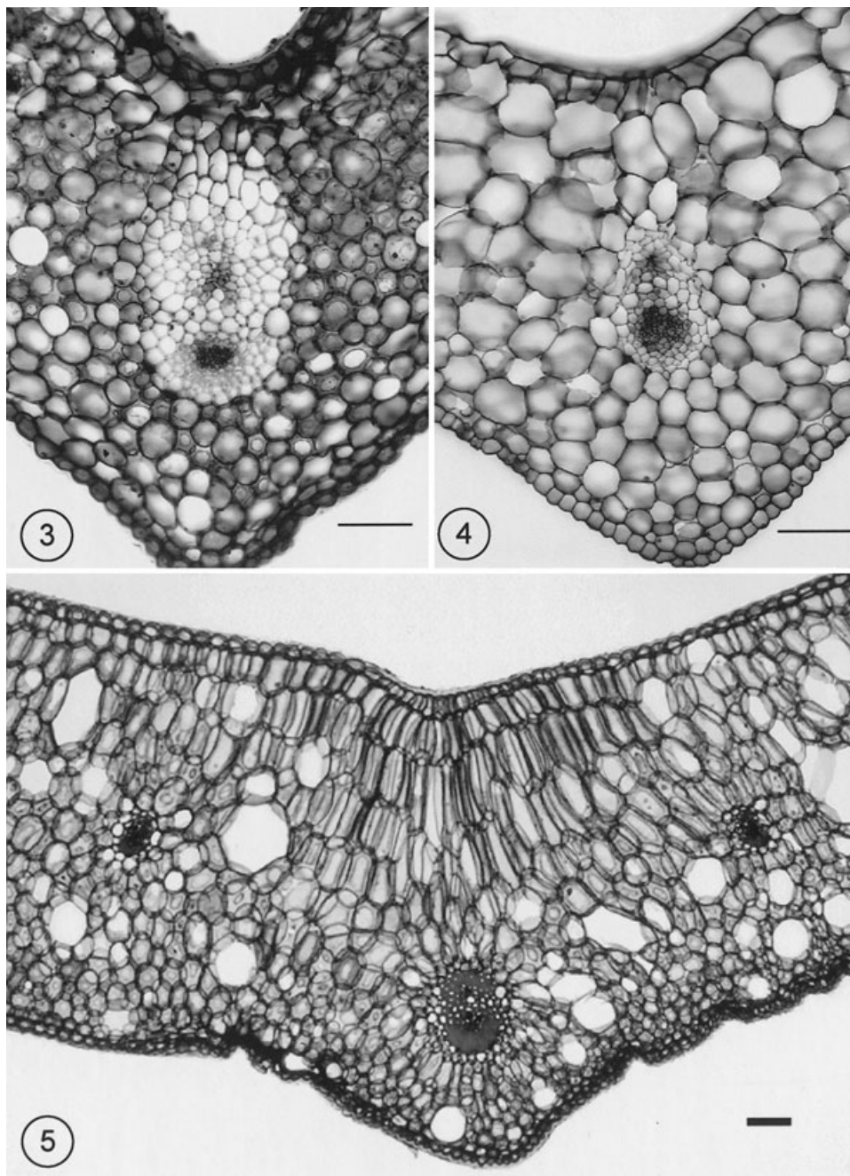
Figures 3–5. Leaf TS showing mesophyll above midrib. Scale bars = 100 \mu\text{m} . Fig. 3. Cribbia brachyceras with mesophyll unmodified. Fig. 4. Rhipidoglossum kamerunense with mesophyll slightly modified. Fig. 5. Angraecum dives showing distinctly modified mesophyll.
