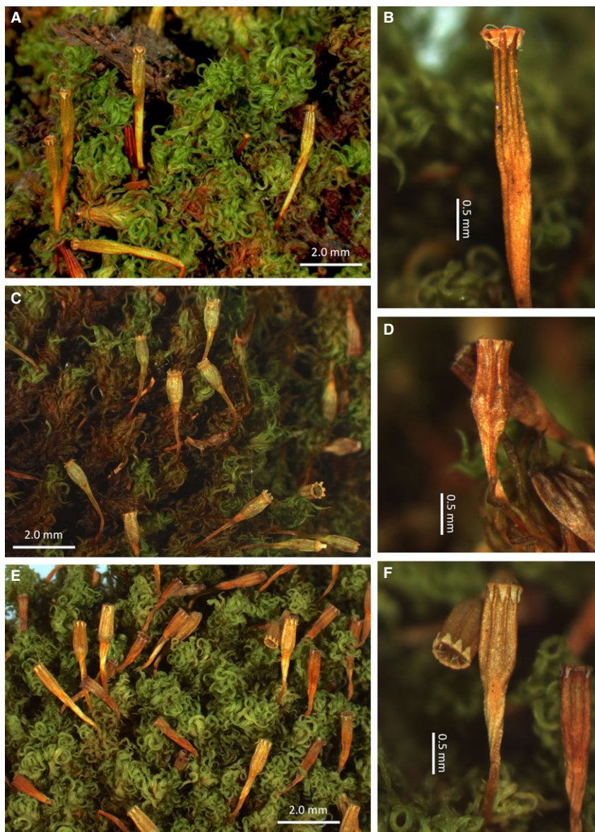
Figure 2. Comparison of general habit and capsule shape when dry and empty of Ulota crispa (A, B; MAUAM-Brio 4441), U. crispula (C, D; MAUAM-Brio 4439) and U. intermedia (E, F; MAUAM-Brio 4749).
