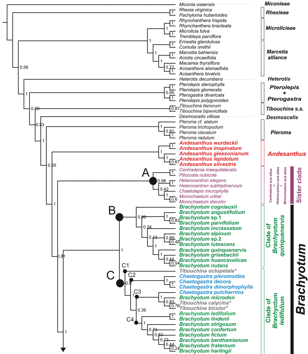
Figure 3. Consensus tree obtained from a Bayesian analysis of the combined nuclear ( waxy +nrETS+nrITS) and plastid ( accd-psal + psbK-psbL + trnS-trnG ) data sets. Posterior probabilities are indicated at nodes. Terminals marked in red are Andesanthus species, in purple are species from the clades of Heterocentron and allies, and Monochaetum and allies, in green are Brachyotum species, in blue are Chaetogastra species, and in grey are species kept as Tibouchina incertae sedis in Guimaraes et al. (2019). Arrows point to species with incongruent positioning. A-F represent the sister group and subclades inside Brachyotum and allies.
