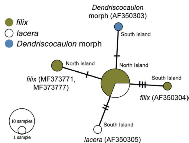
Figure 1. ITS haplotype network of the Sticta filix-lacera complex in New Zealand. Tick lines indicate number of base call differences between haplotypes.
